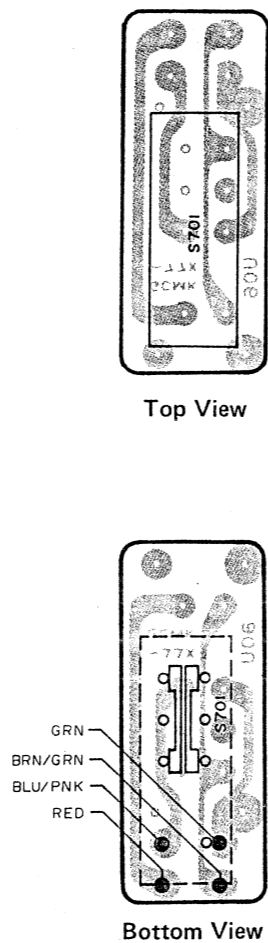
Timer Switch P.C. Board
