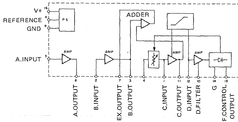
NE645N: OC101, 102, 103, 104
