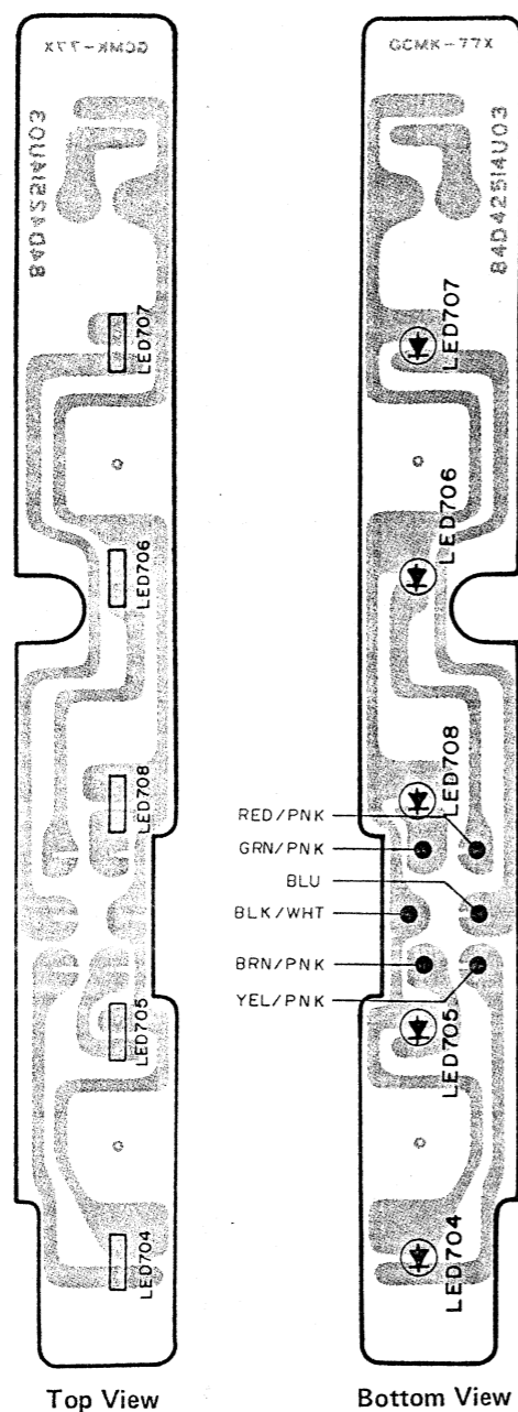
Keyboard Indicator P.C. Board
