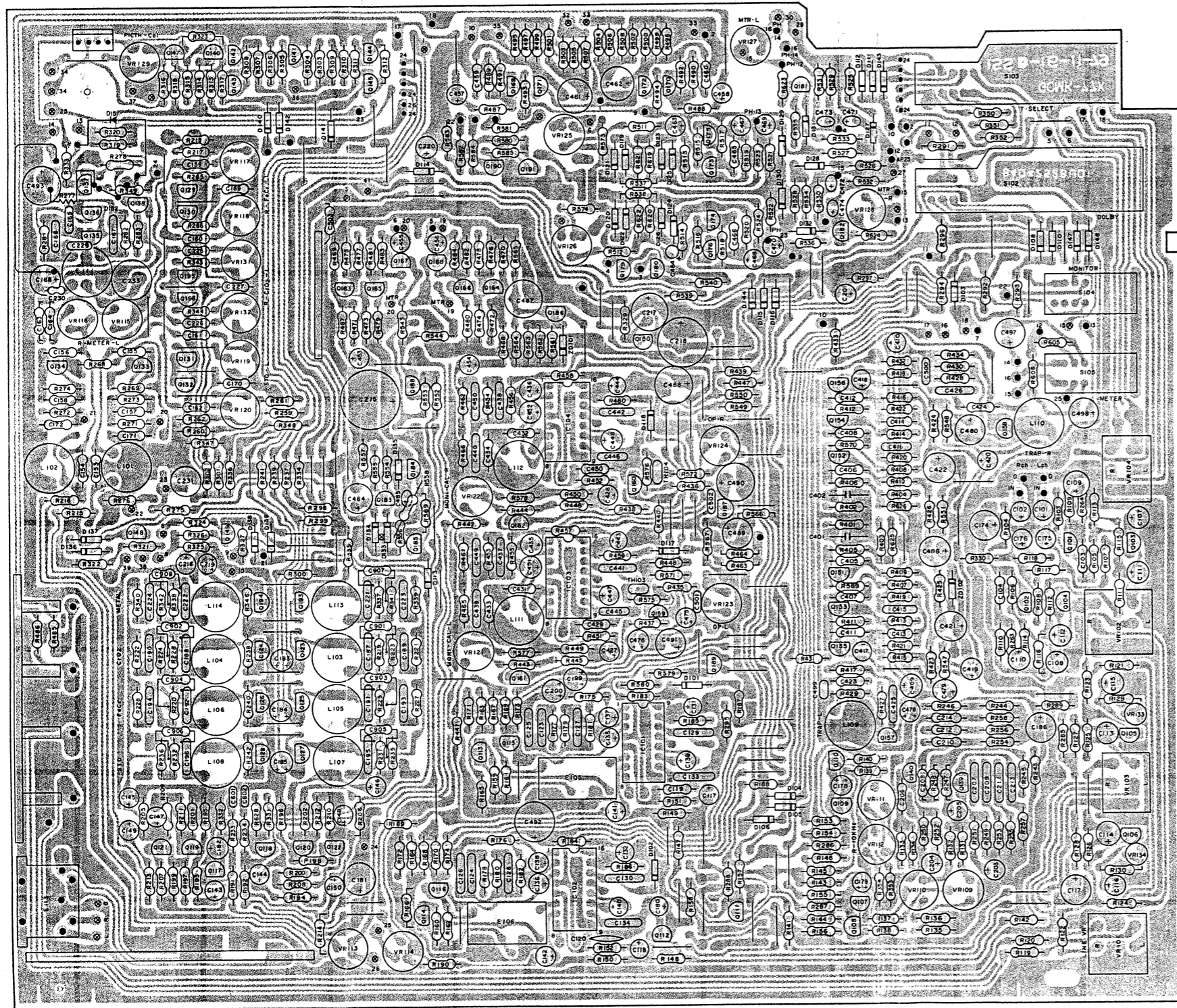
Top View
