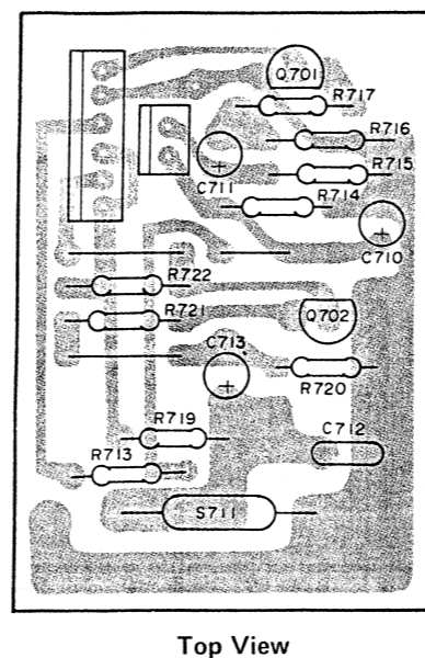
Shut Off P.C. Board
