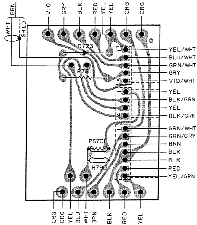
Bottom View
