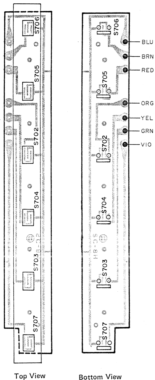
Keyboard P.C. Board
