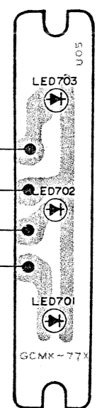
Bottom View
