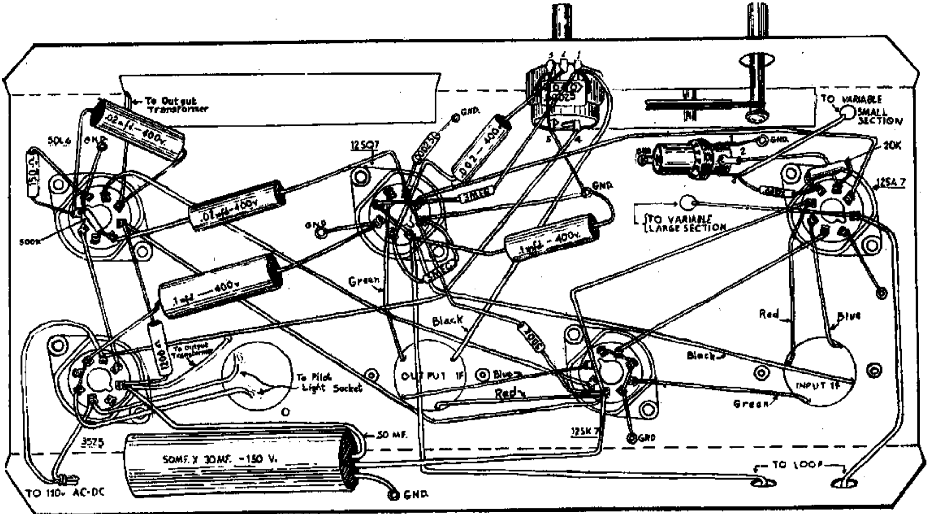
PICTORIAL DIAGRAM OF MODEL S-5C
