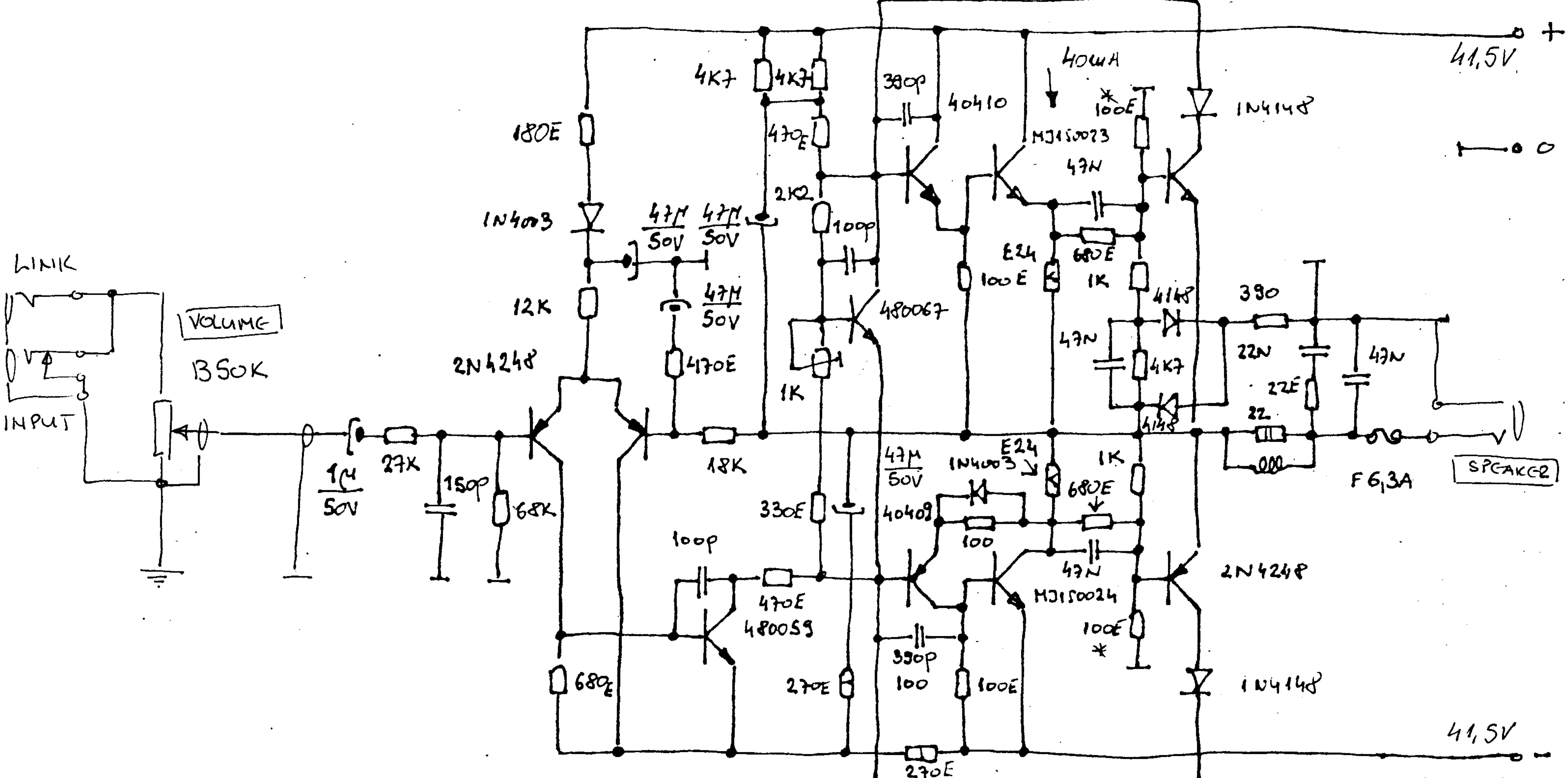
Acoustic control corp model 215B-120 drawing by VintageKiki
