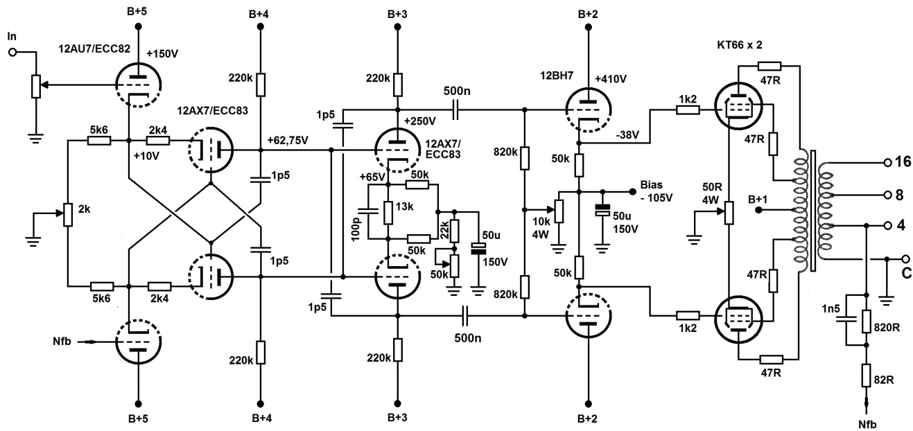
Golden Ear Laboratory Amplifier by Joseph Marshall 1956
