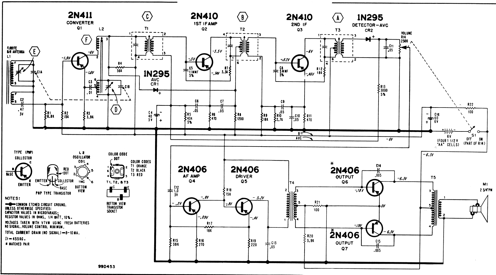
Figure 7. Schematic of 7V1 Chassis.
