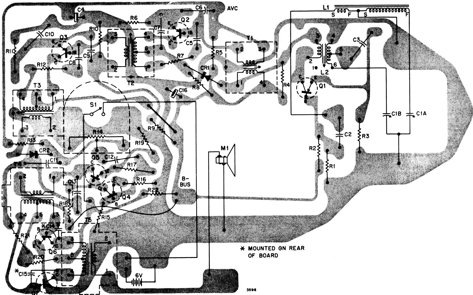
Figure 8. Rear View of Etched Circuit Board Used in 7V1 Chassis. Gray area represents etched wiring; black symbols and lines represent components and connections on opposite side.
