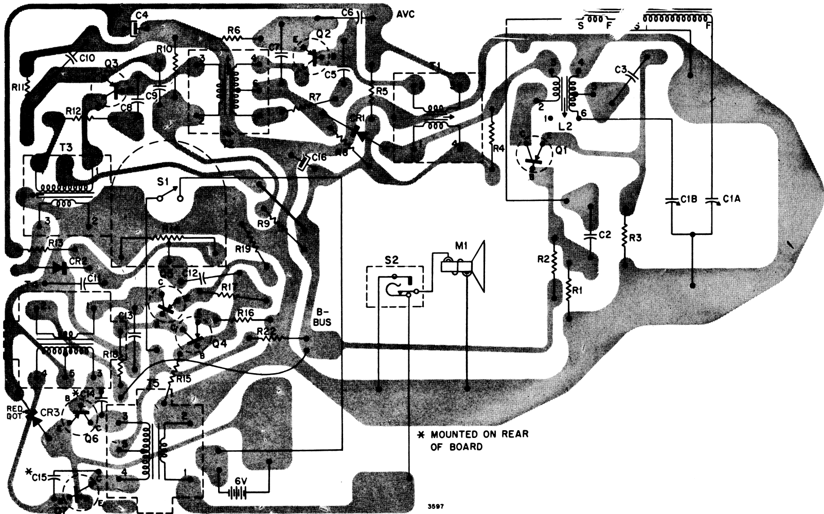
Figure 10. Rear View of Etched Circuit Board Used in 7V1A and 7V1B Chassis. Gray area represents etched wiring; black symbols and lines represent components and connections on opposite side.
