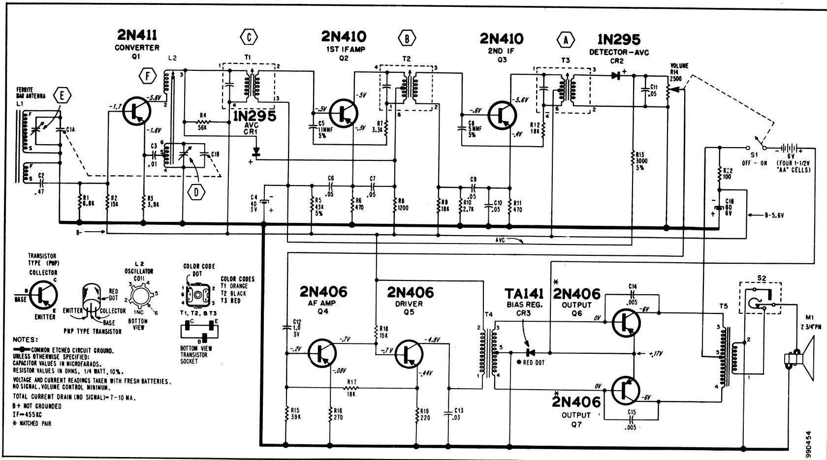
Figure 9. Schematic of 7V1A and 7V1B Chassis.
