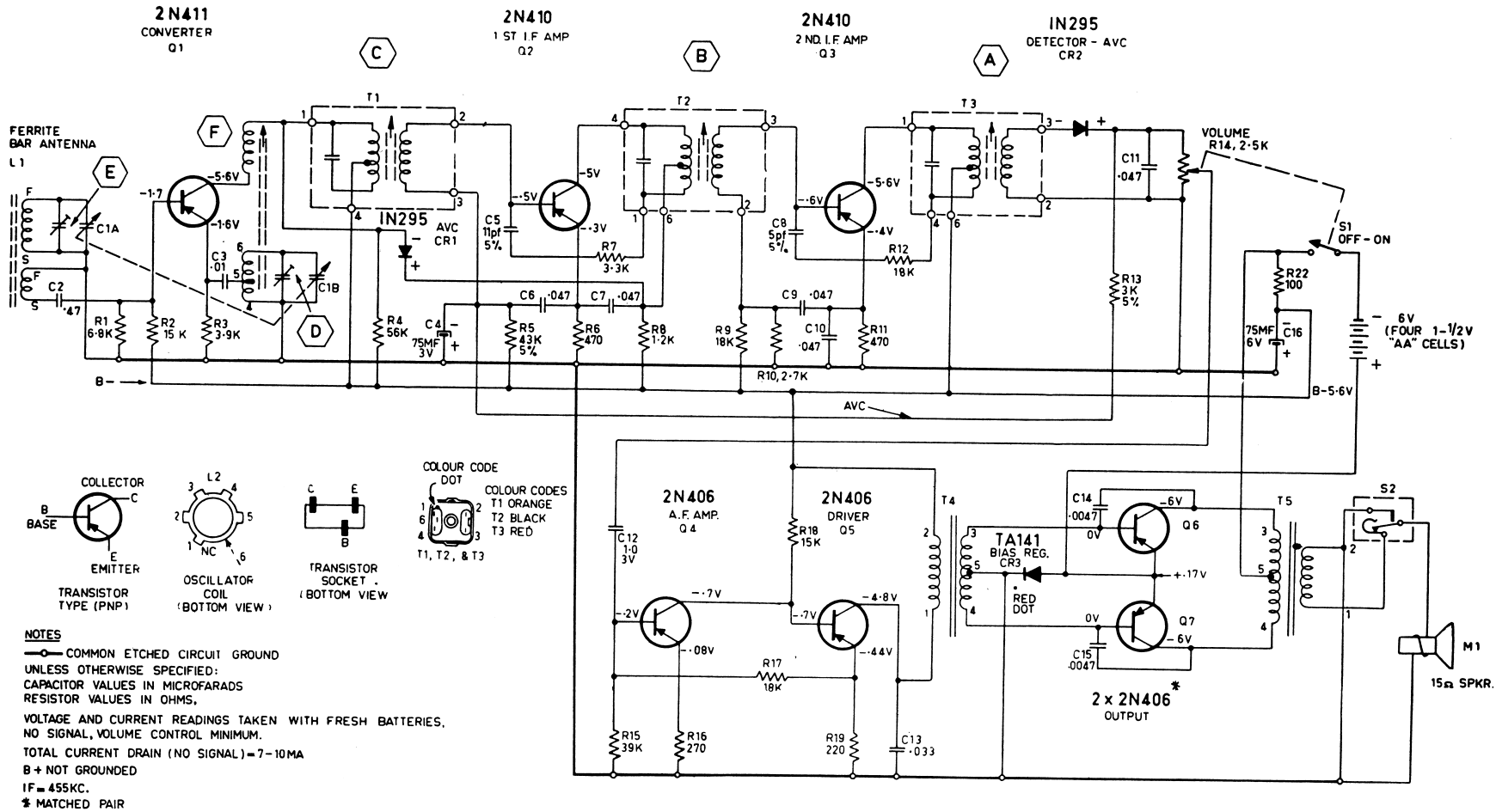
Figure 6. Schematic of 7V2 Chassis.
