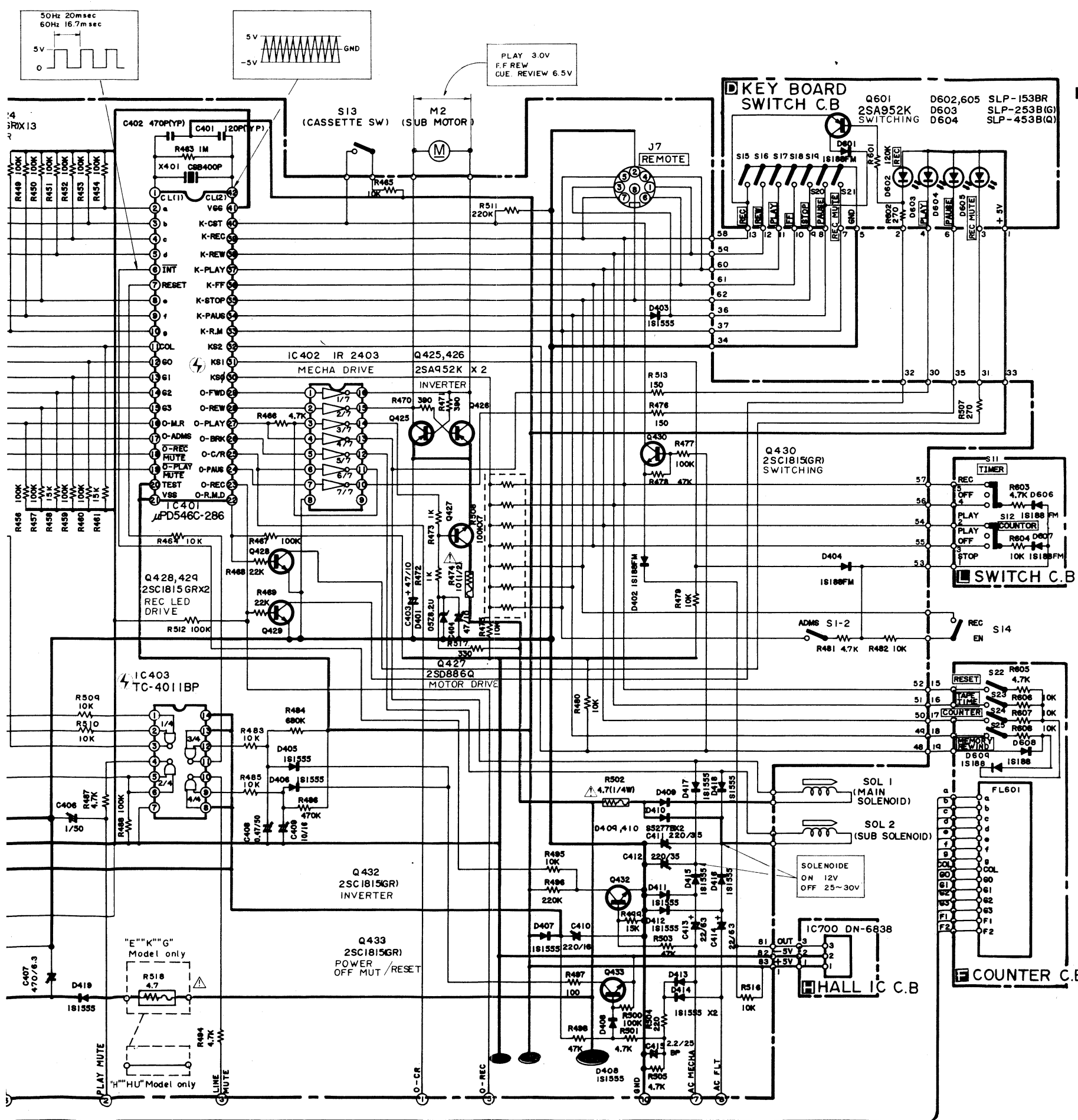
MECHA MODE and OUTPUT of MPU
