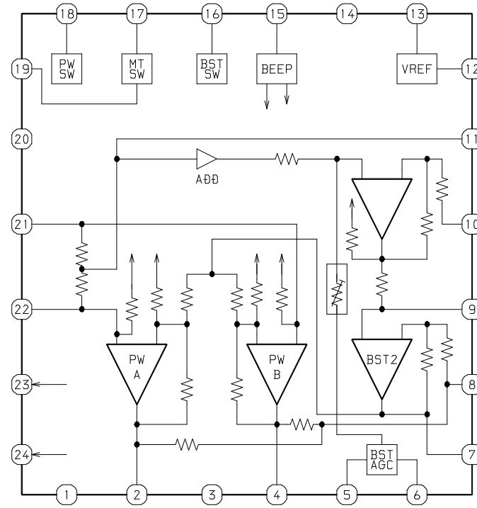
IC, TA2131FL
