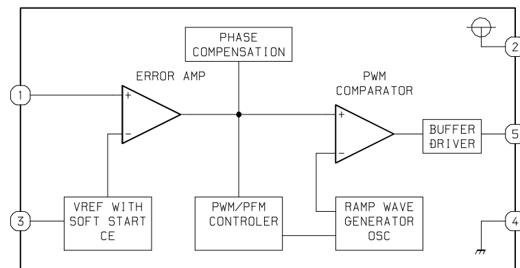
IC, XC6367B102MR
