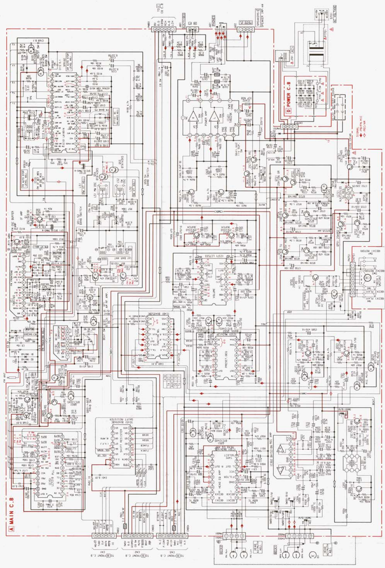
SCHEMATIC DIAGRAM - 1 (MAIN SECTION : HE, HR)
