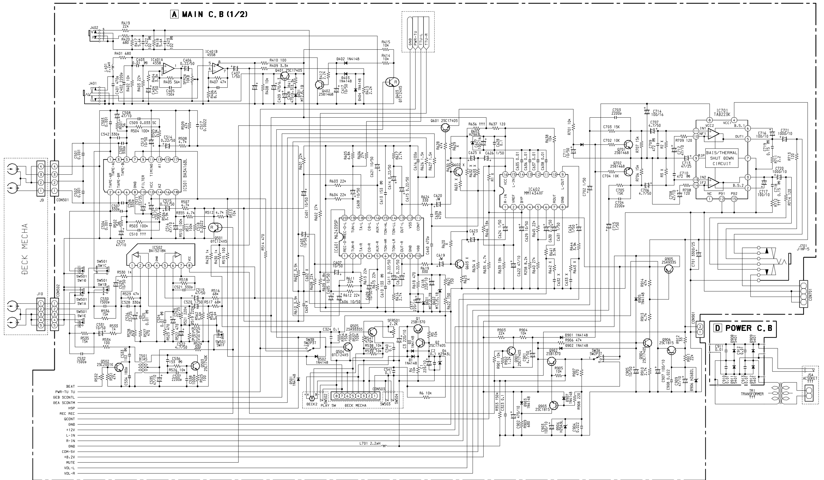
SCHEMATIC DIAGRAM – 1 (MAIN 1/2)
