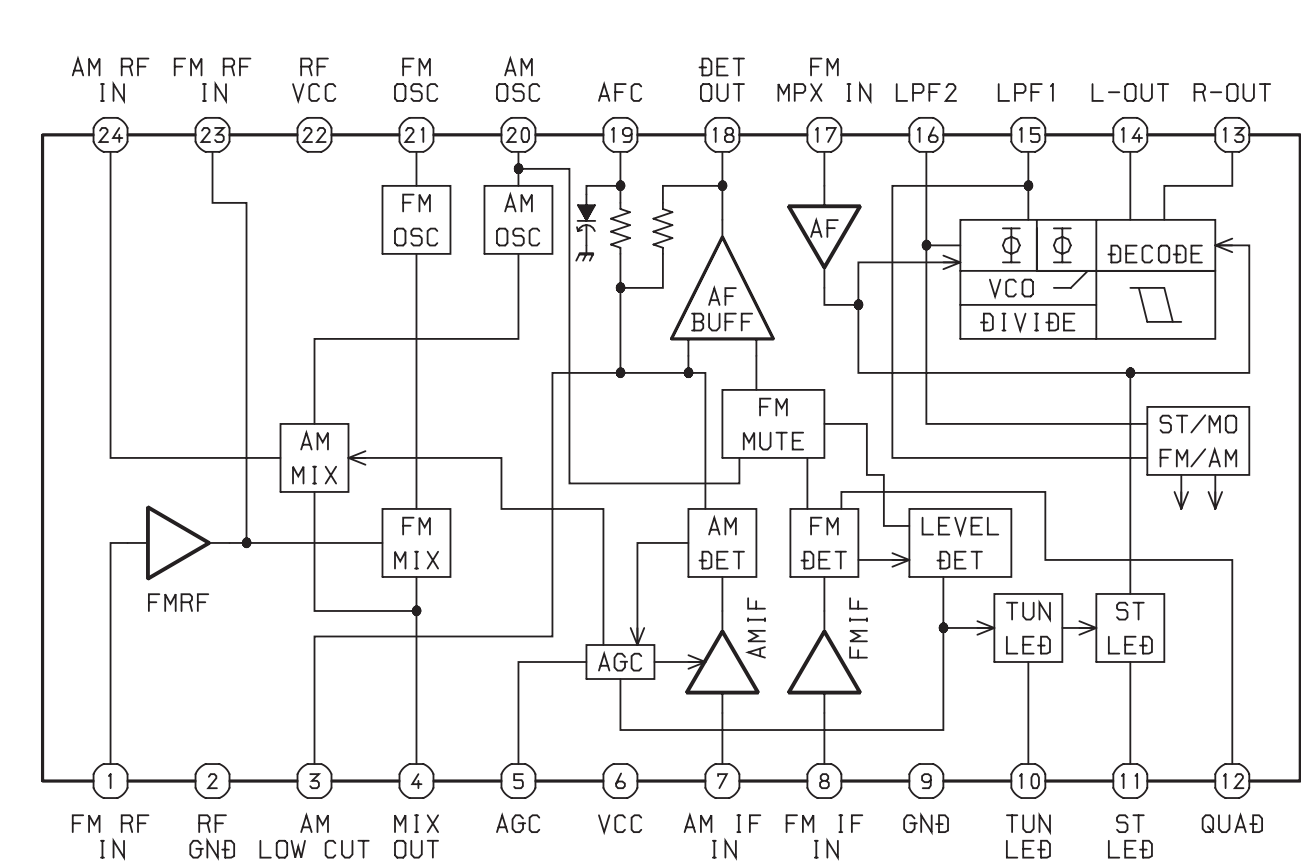
IC BLOCK DIAGRAM IC, TA2111FN
