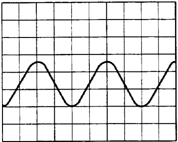
① U1 Pin 66 (EXTAL) VOLT/DIV: 1V TIME/DIV: 20nS
