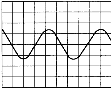
⑨ CN1 Pin 26 (L OUT) VOLT/DIV: 1.0V CN1 Pin 28 (R OUT) TIME/DIV: 0.2mS 1kHz OUTPUT
