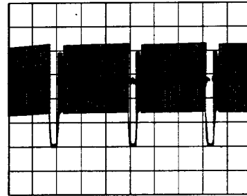
BLUE VOLT/DIV: 100mV TIME/DIV: 20μS
