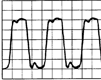
⑥ U14 Pin 66 (VD CLK) VOLT/DIV: 1V TIME/DIV: 20nS
