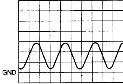
⑤ U12 Pin 6 (SC IN) VOLT/DIV: 1.0V TIME/DIV: 0.1μS
