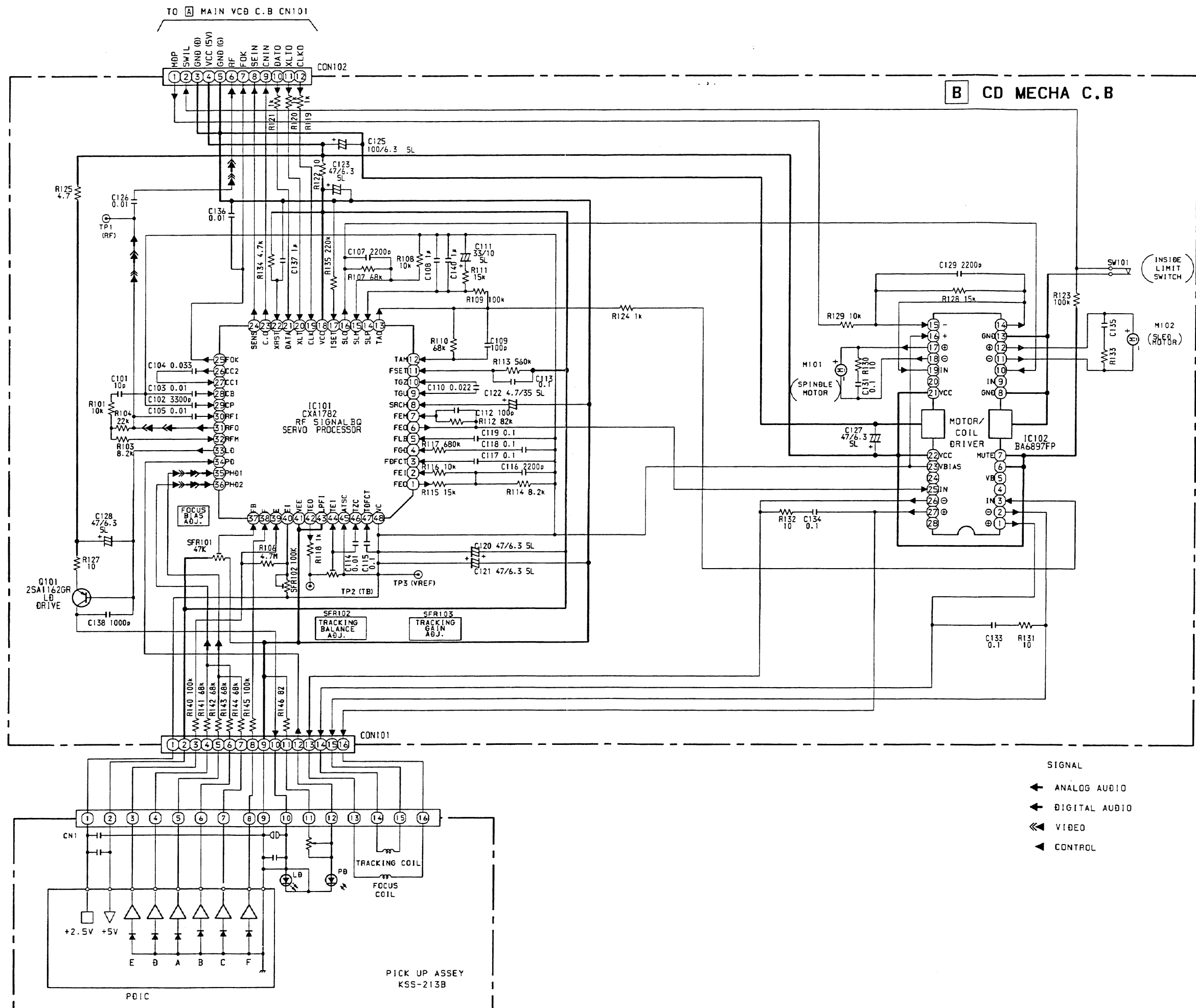
SCHEMATIC DIAGRAM-1 (CD MECHA)
