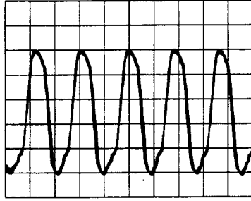
⑦ U14 Pin 135 (CLK) VOLT/DIV: 1V TIME/DIV: 20nS
