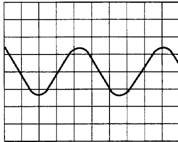
⑨ CN1 Pin 26 (L OUT) VOLT/DIV: 1.0V CN1 Pin 28 (R OUT) 1kHz OUTPUT TIME/DIV: 0.2mS
