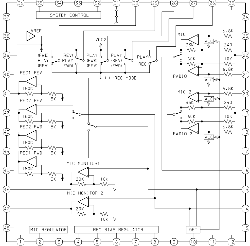
IC, LA3235W
