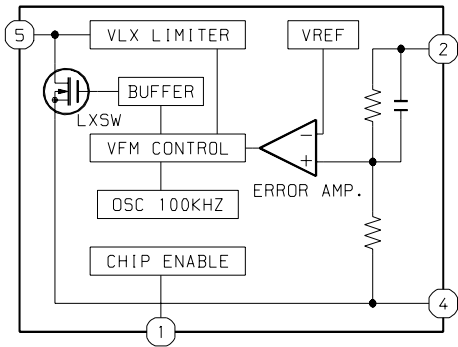
IC, RN5RK241A
