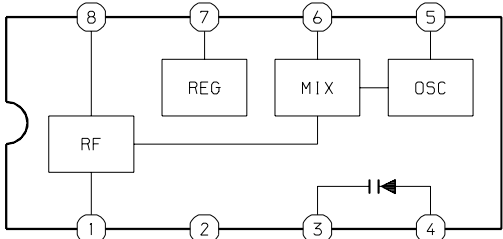
IC, TA7371AF
