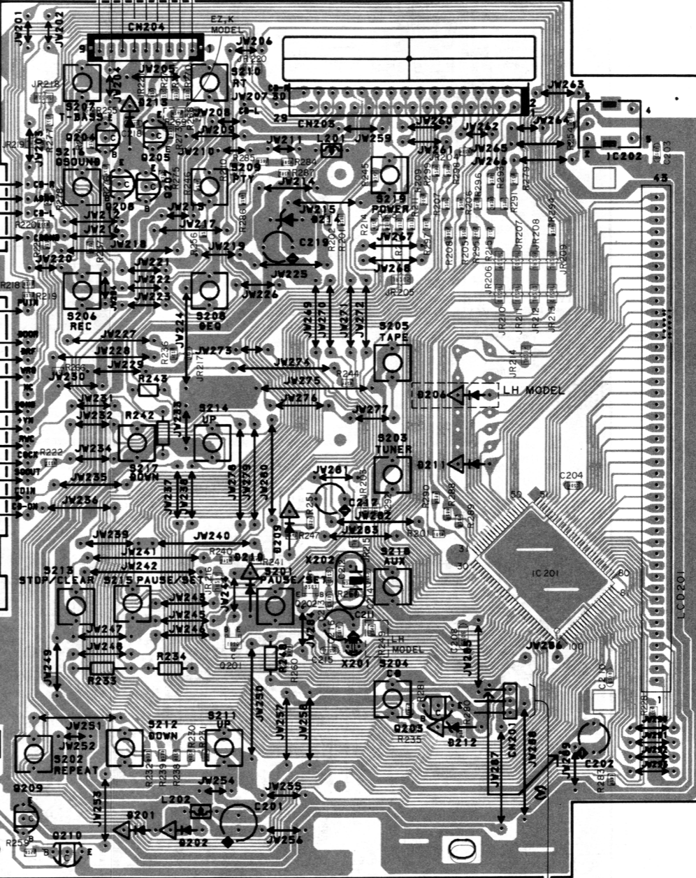
C FRONT C.B
