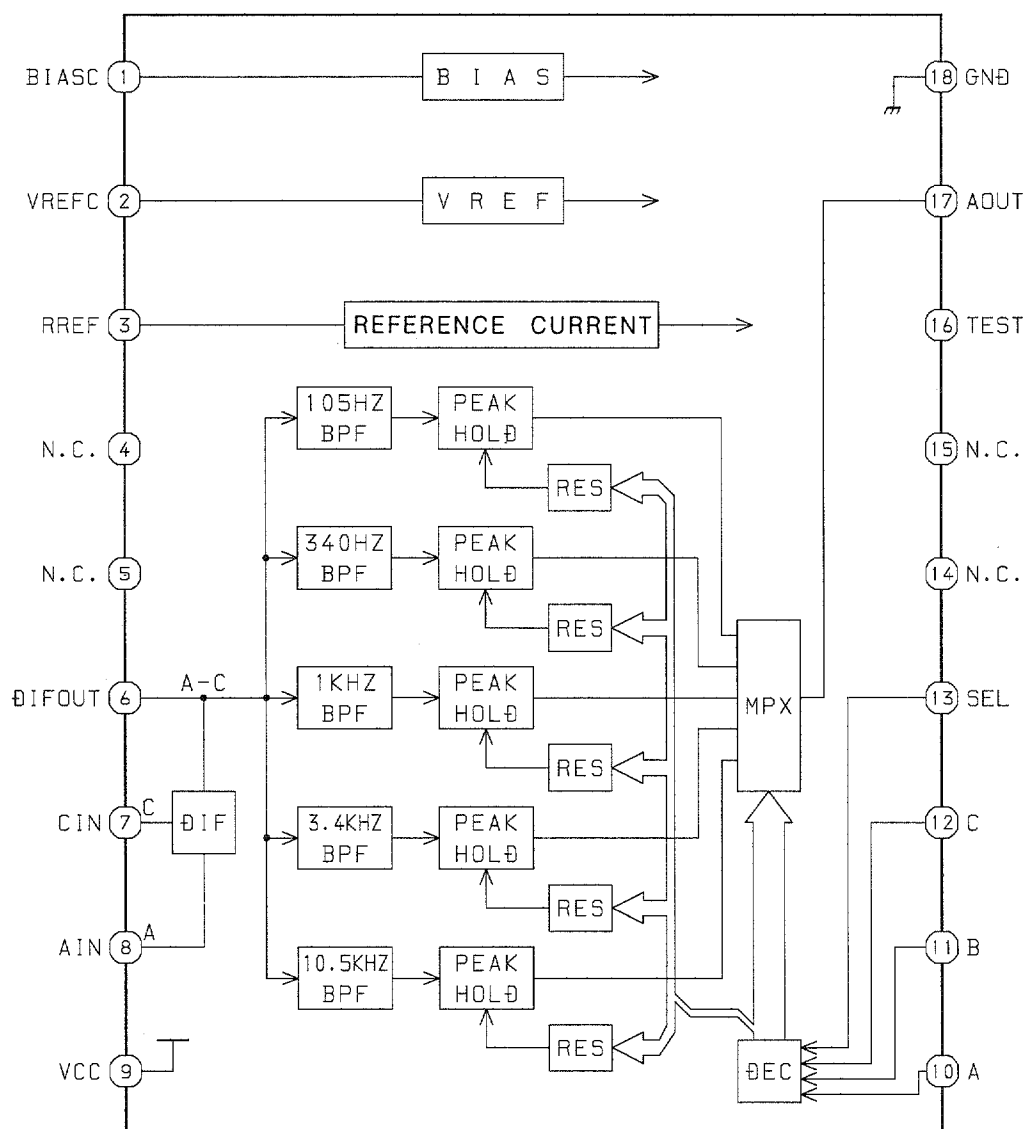
IC, BA3835S
