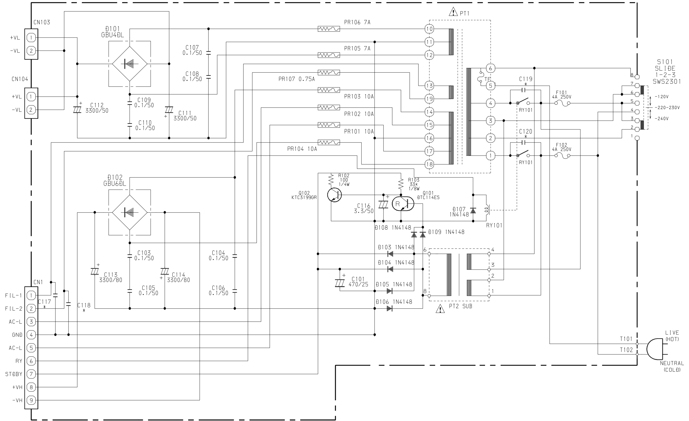
SCHEMATIC - PT
