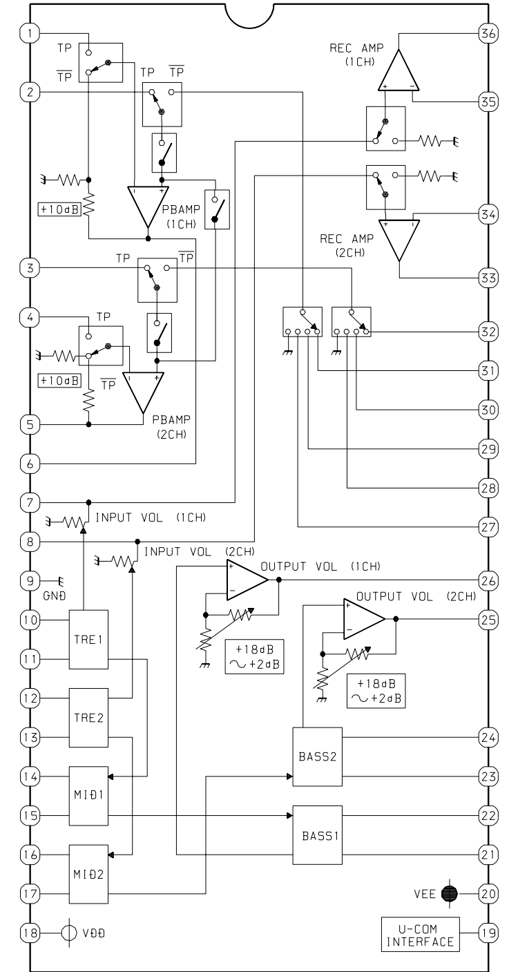
IC, M61518FP
