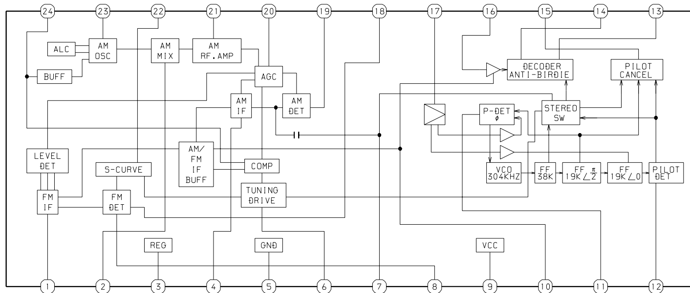
IC, LA1845L
