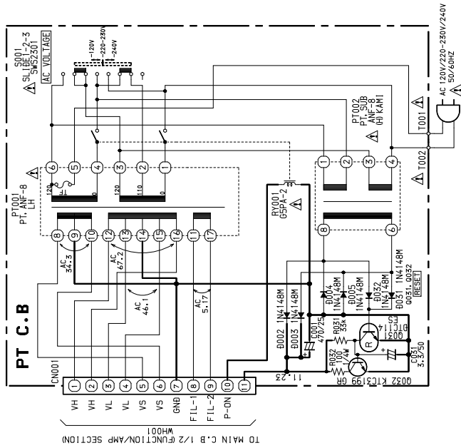
SCHEMATIC DIAGRAM-7 [PT SECTION] <50HA>
