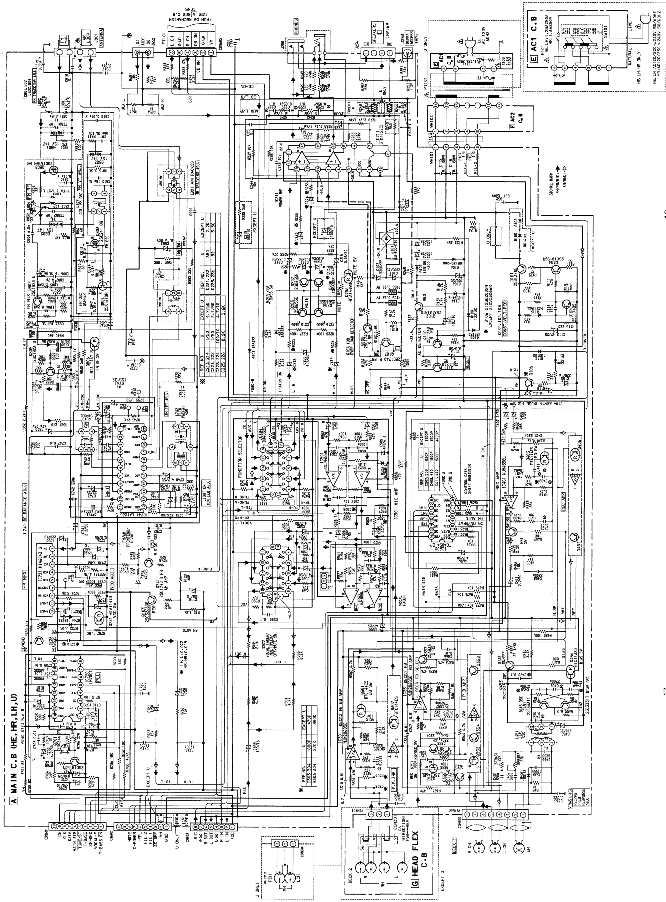
SCHEMATIC DIAGRAM - 1 (MAIN : HE, HR, LH, U)
