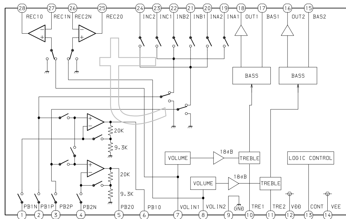
IC, BD3881FV
