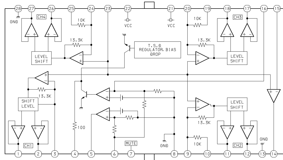
IC, BA5826FP
