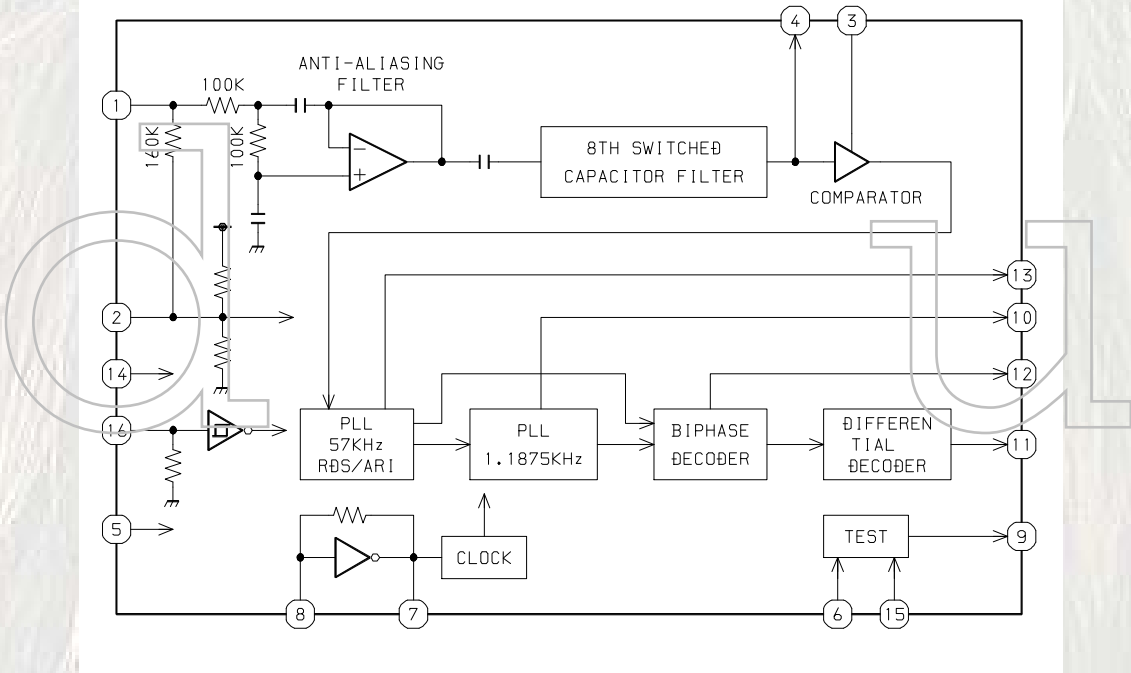
IC, BU1920FS
