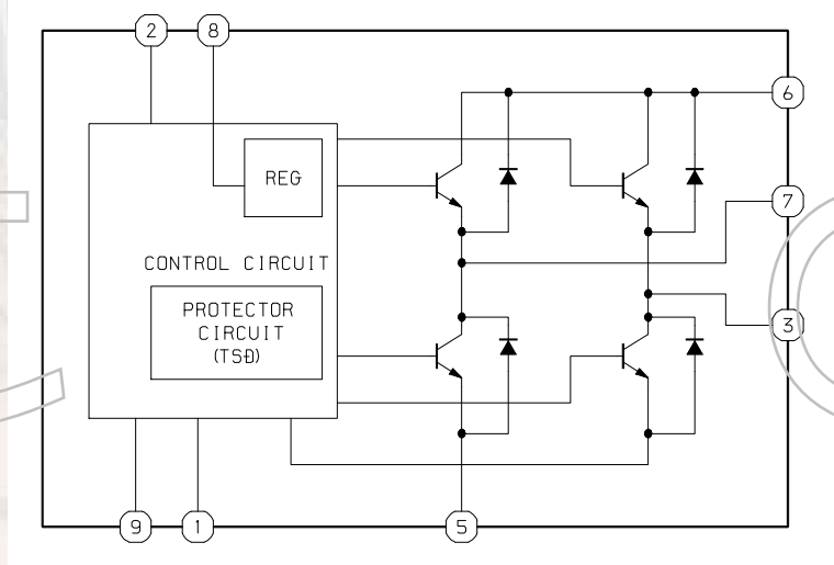
IC, TA7291S
