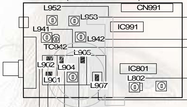
TUNER C.B (COMPONENT SIDE)
