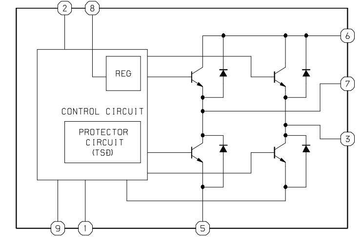
IC, TA7291S
