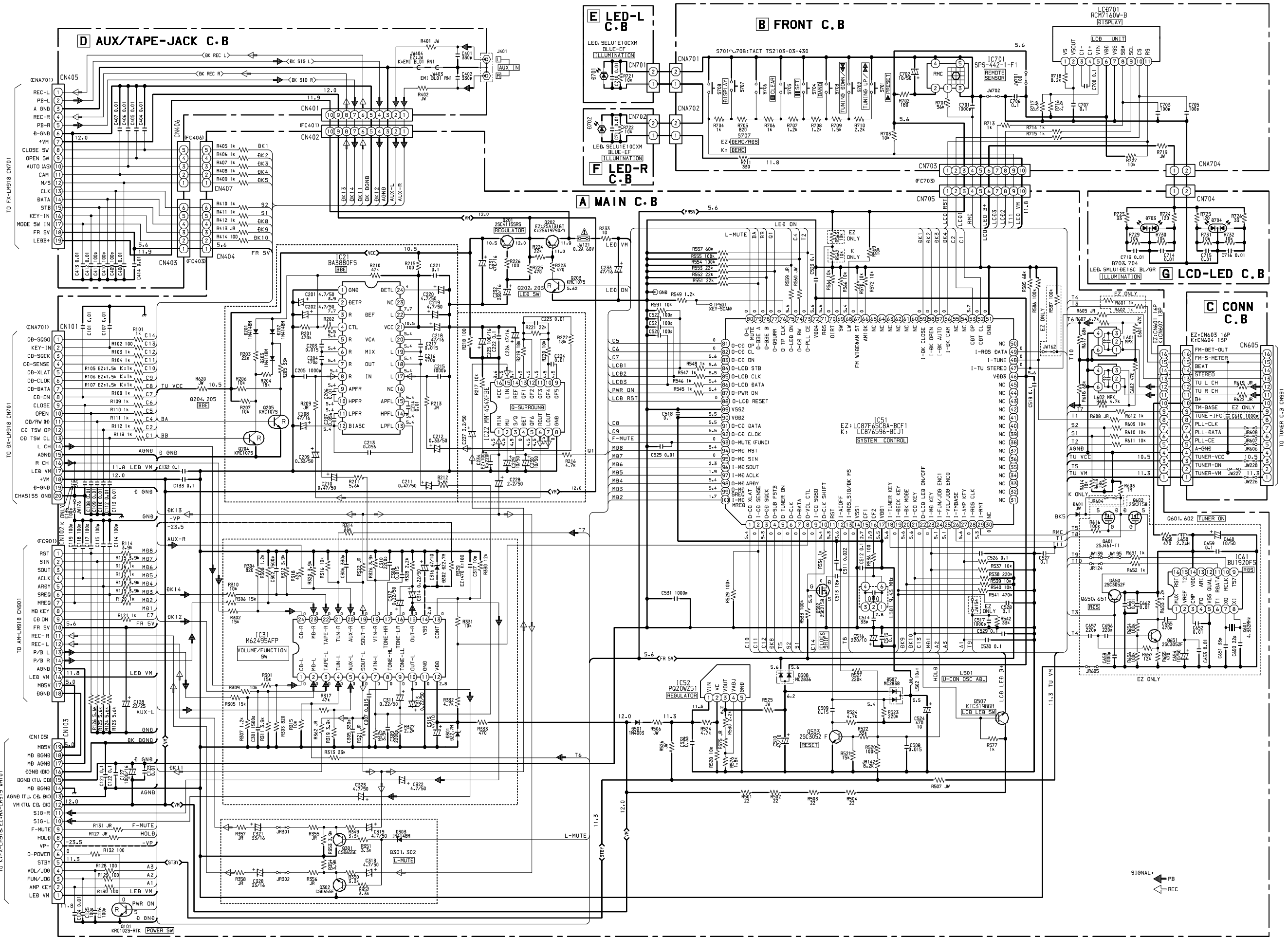
SCHEMATIC DIAGRAM - 1 (MAIN / FRONT / CONN / AUX / TAPE - JACK / LED - L / LED - R / LCD - LED)
