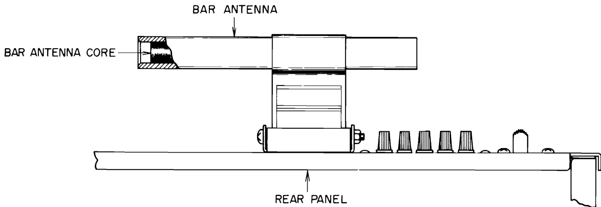
Fig. 5 Model AA-1020
