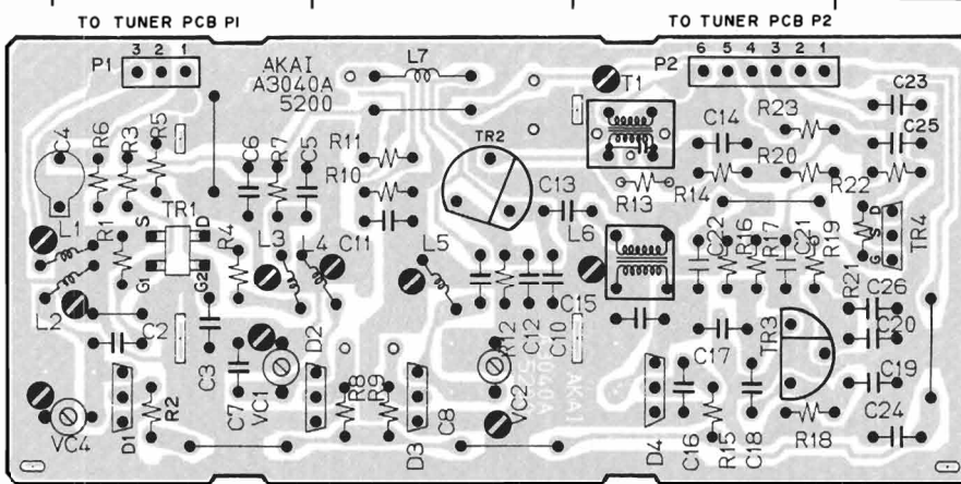
FRONT END PCB A3040C 5200
