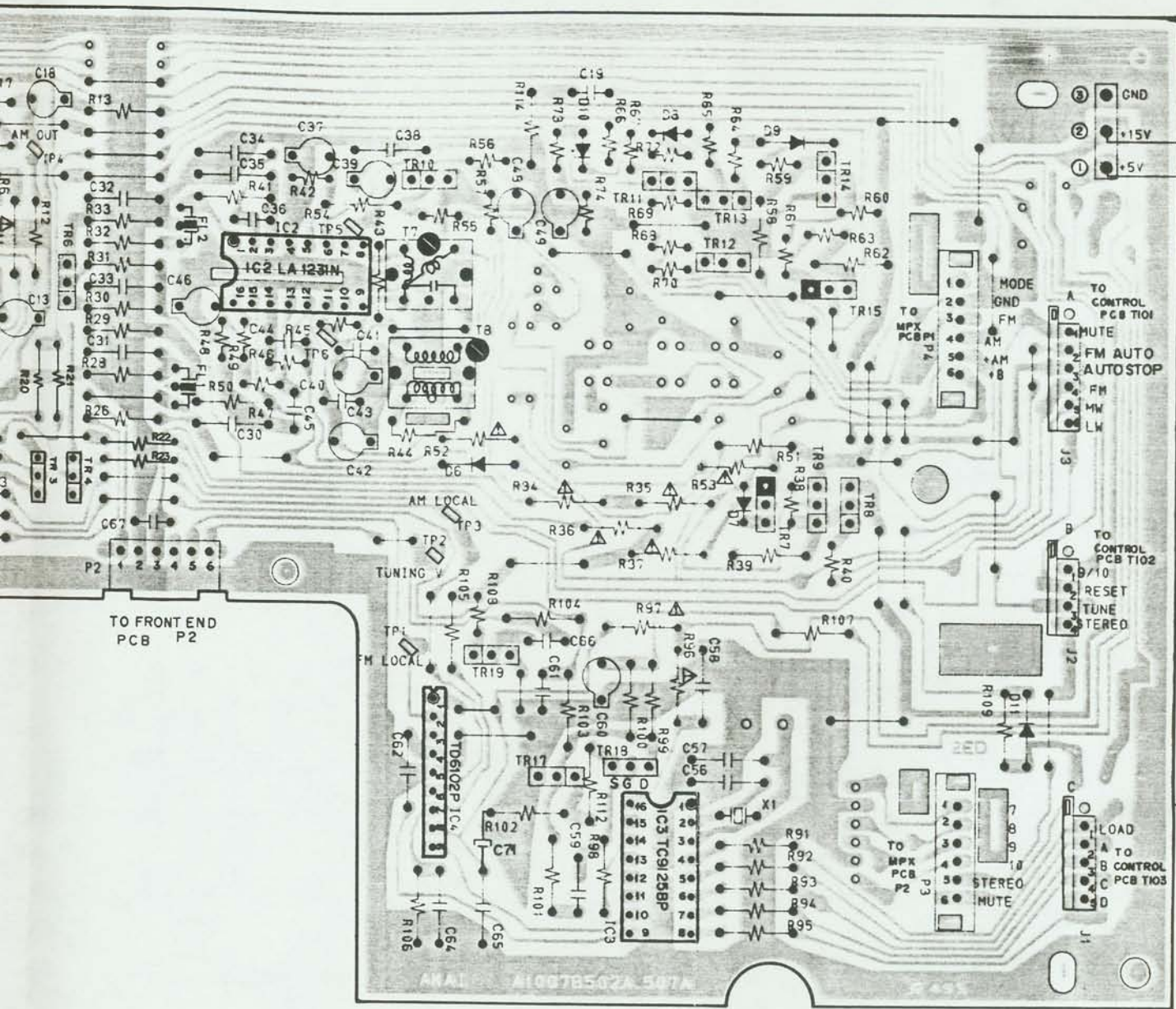
TUNER PCB A1007B507A (2ED) [B][E]
