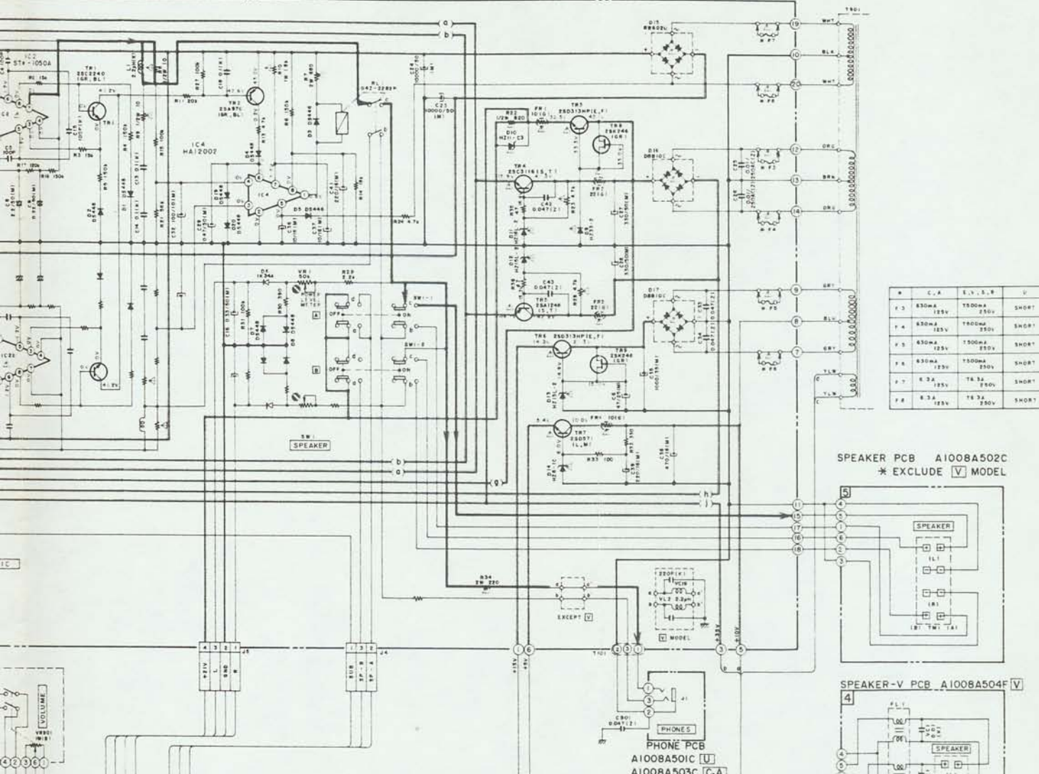
POWER PCB A1008A503E
