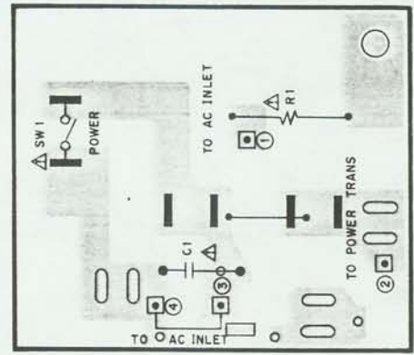
POWER PCB A1008A503E C A
