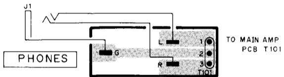
PHONE PCB A1008A501C U A1008A503C C, A
