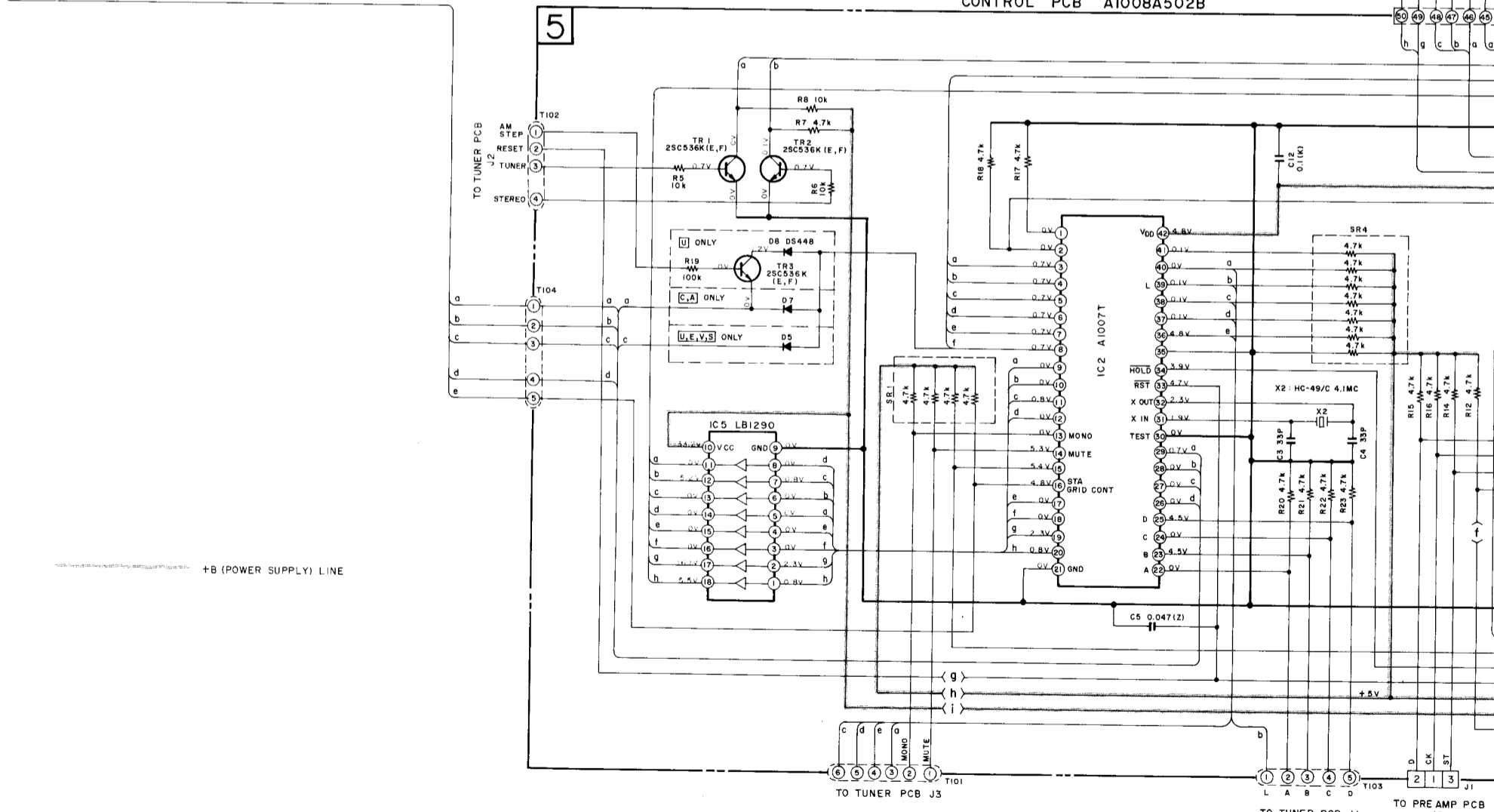
CONTROL PCB A1008A502B
