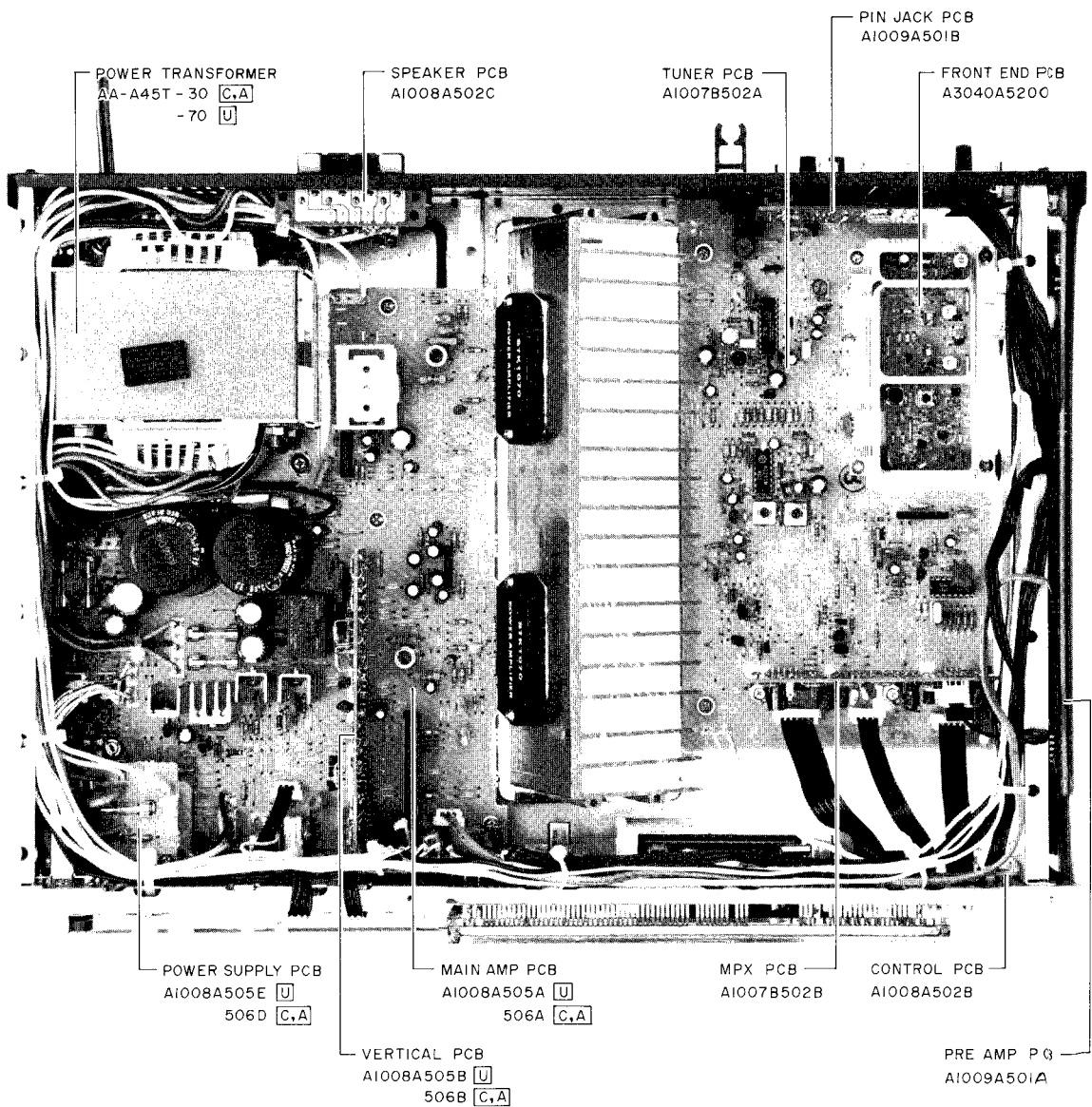
Fig. 4-2 Top View
