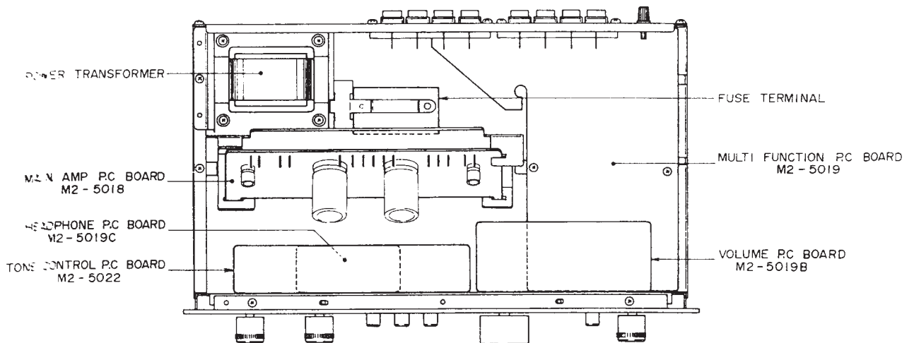
Fig. 2 Top View
