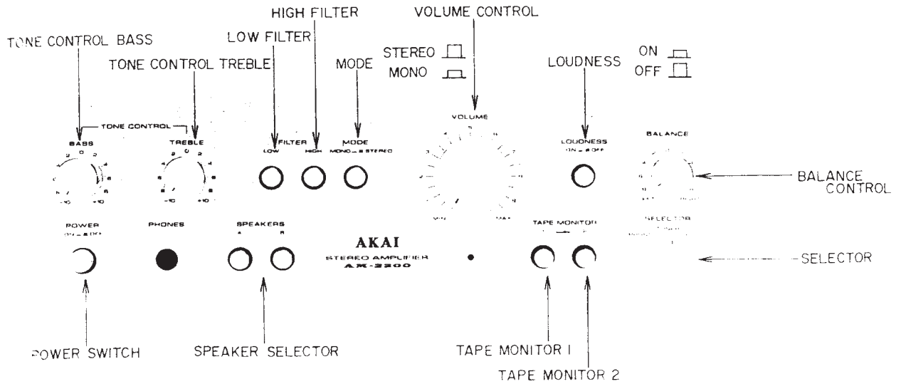
Fig. 1 Controls
