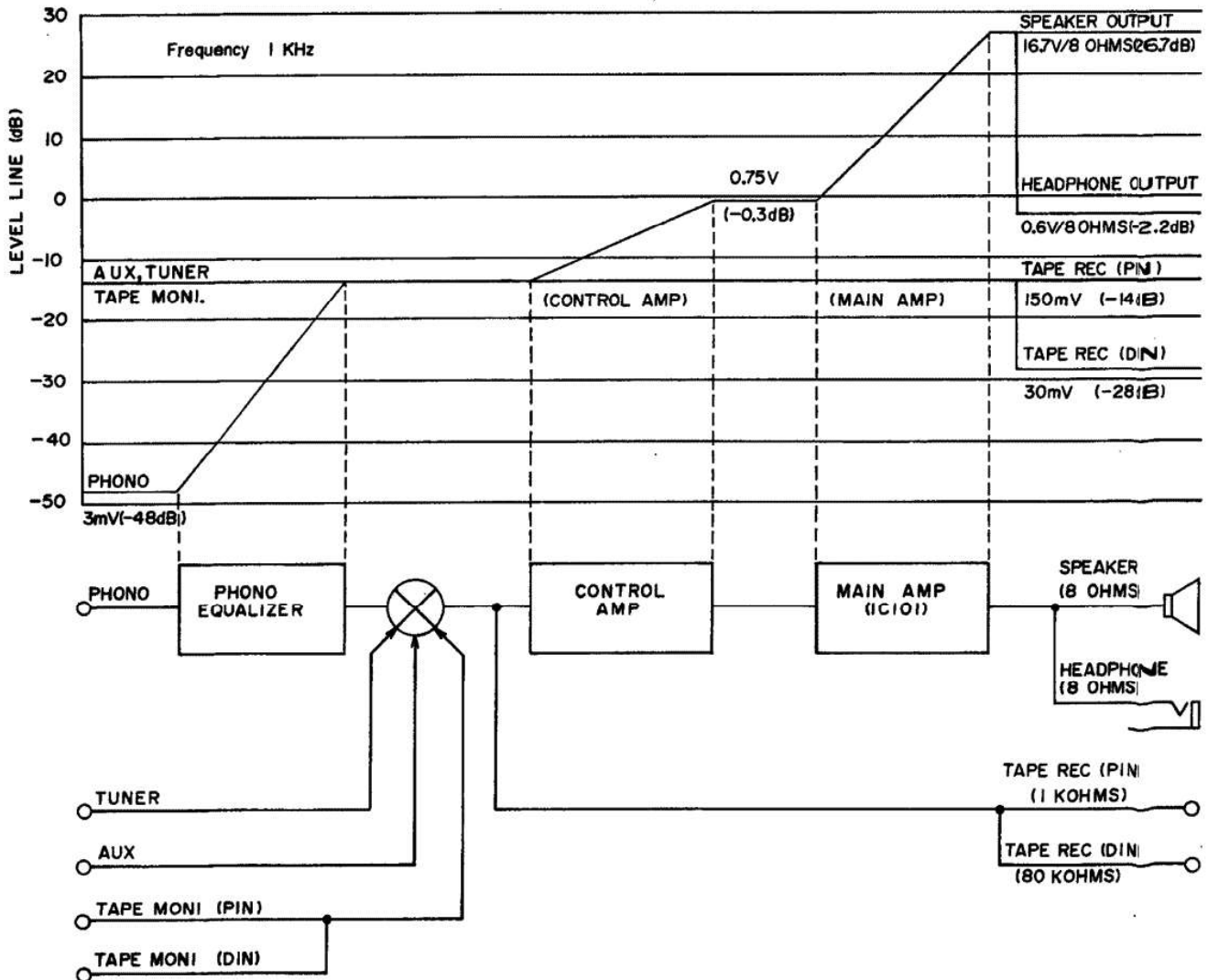
Fig. 5 Level Diagram.
