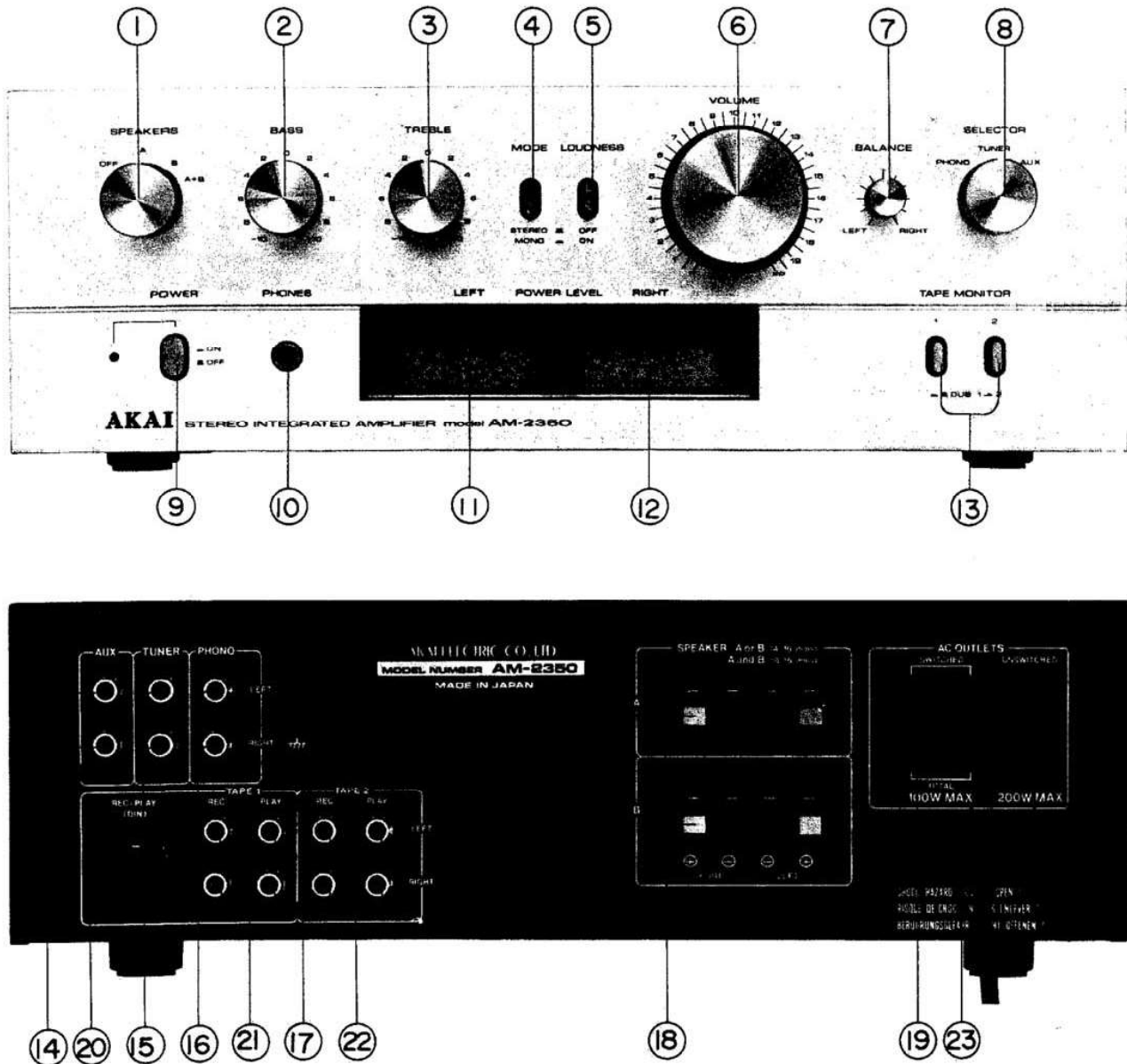
Fig. 1 Front and Rear Panel Controls.
