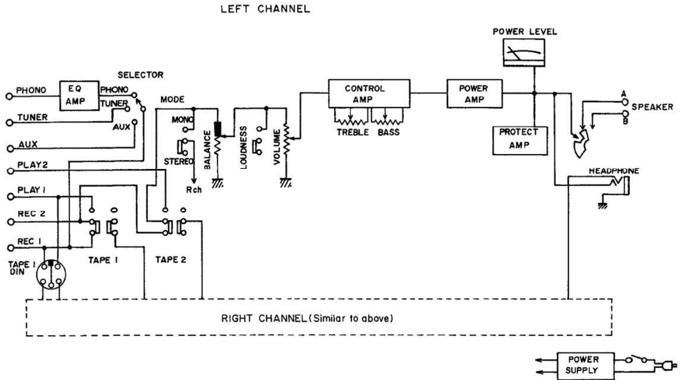
Fig. 4 Block Diagram.
