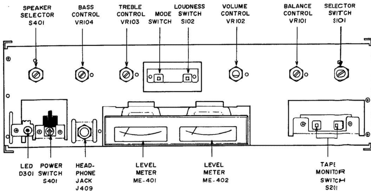
Fig. 3 Front View.
