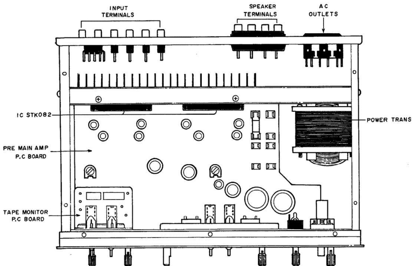
Fig. 2 Bottom View.
