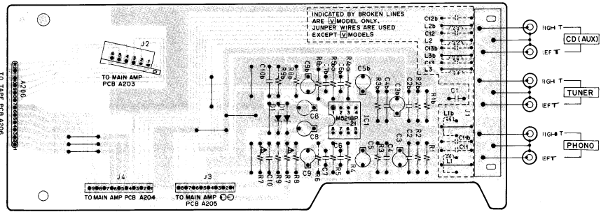
EQUALIZER PCB A2033A501B [U] 4502B [C,A] 4503B [E,B,S] 4504B [V]
