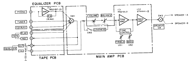
AM-A1 BLOCK DIAGRAM NO. 840801A
