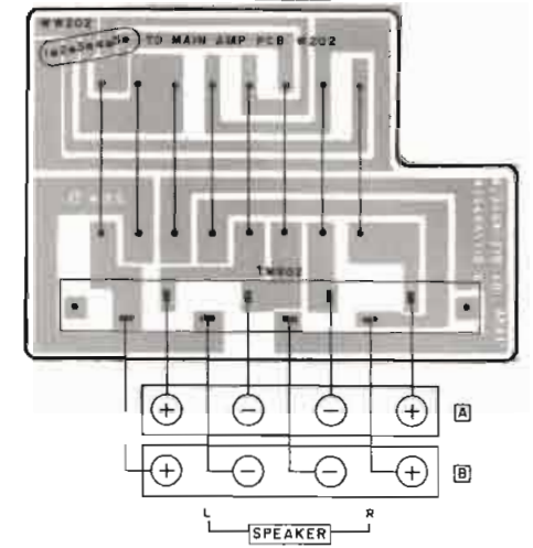
SPEAKER TERMINAL PCB A2040A501B U 502B C.A 503B E.B.S
