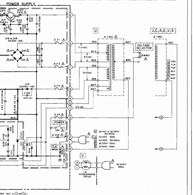
(TUNER) AT-M5 SCHEMATIC DIAGRAM No. 830212A
