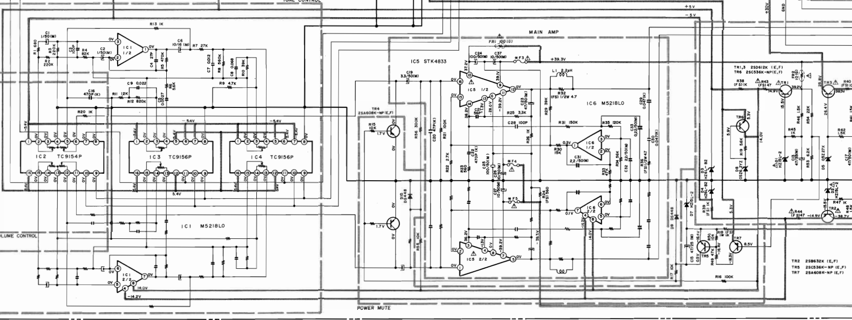
AM-M5 MAIN AMP PCB A2024A5010(U) A2024A5011(C) A2024A5012(E)
