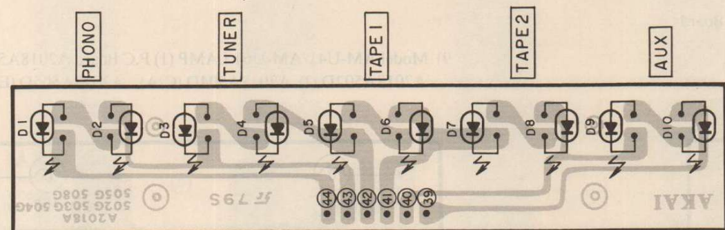
LED(1) PCB (U) A2018A503G (J)A2018A502G (C,A)A2018A504G (E,V,B,S)A2018A505G
