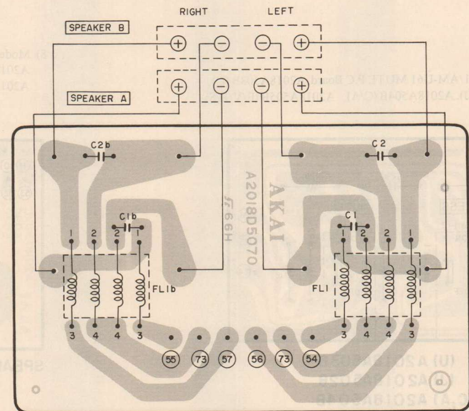
TERMINAL PCB A2018D5070
