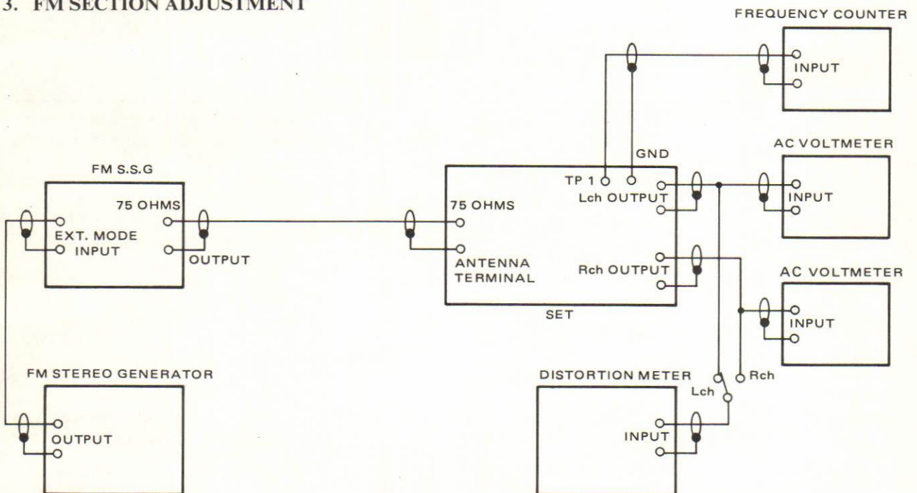
Fig. 13 Instruments Connection for FM Section Adjustment
