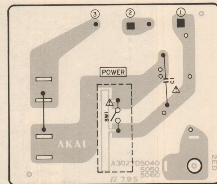
POWER PCB A3027D5040
