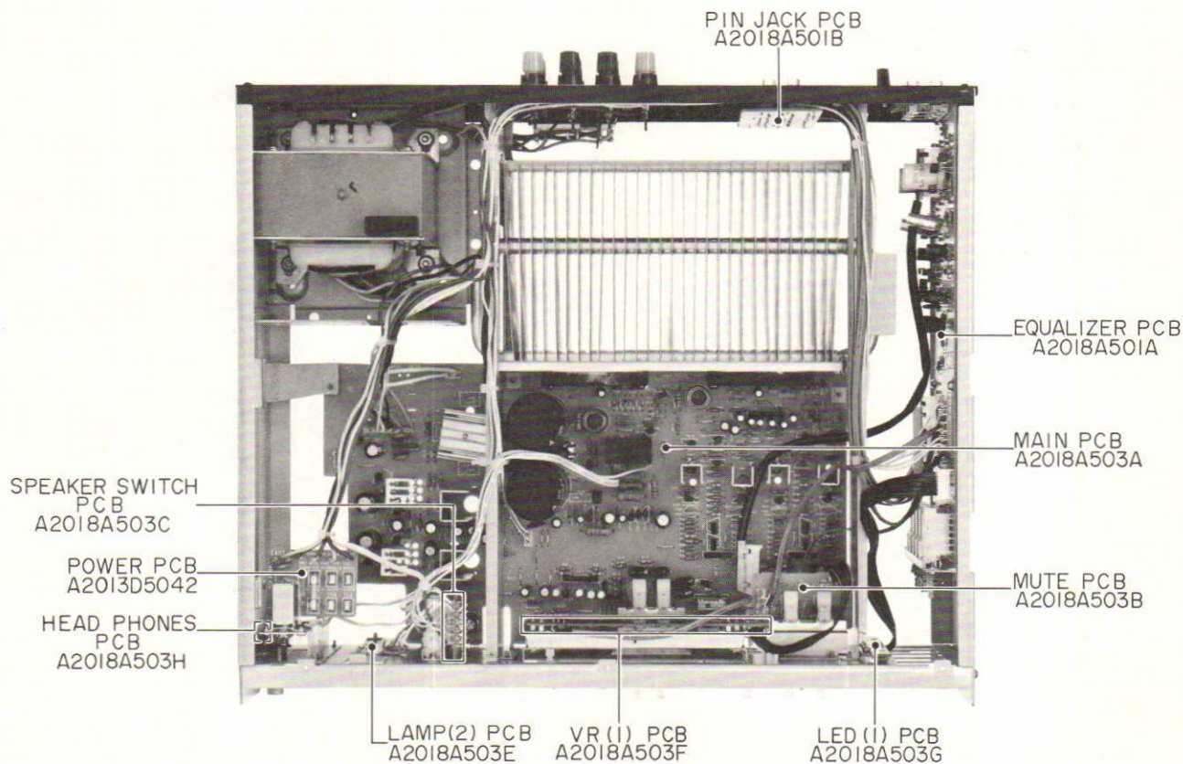
Fig. 4 Top View
