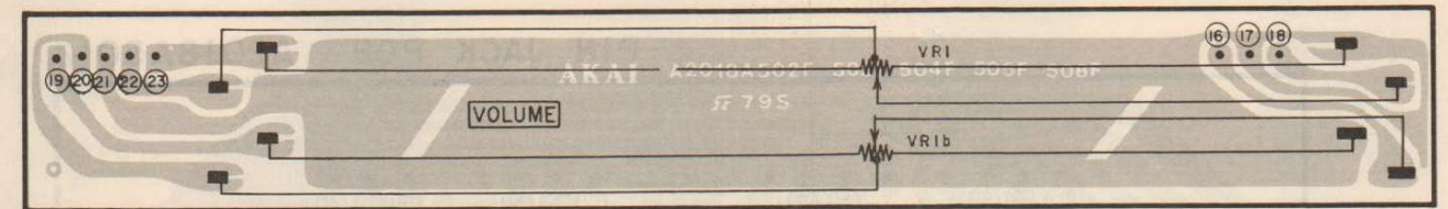
VR (1) PCB (U)A2018A503F (J)A2018A502F (C,A) A2018A504F (E,V,B,S)A2018A505F
