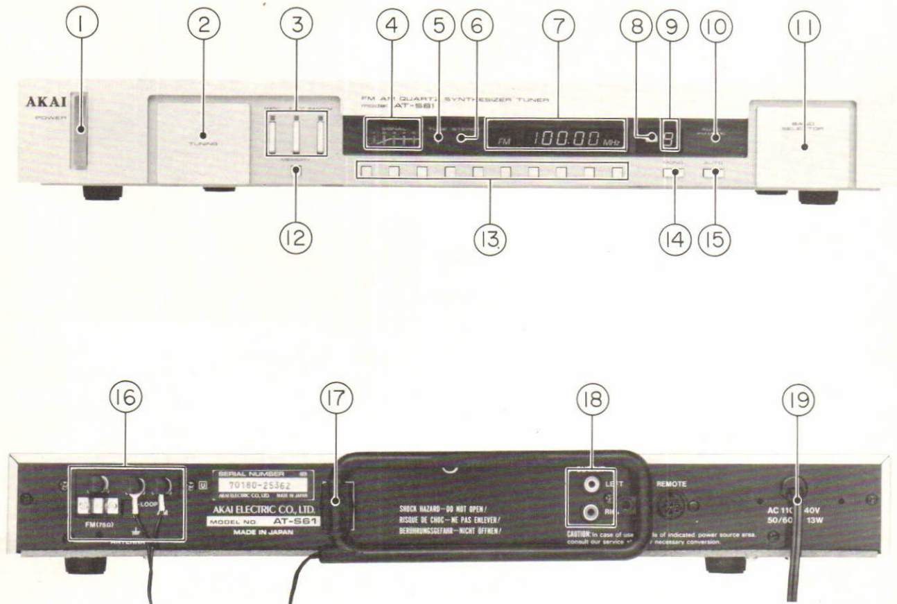
Fig. 1 Controls
