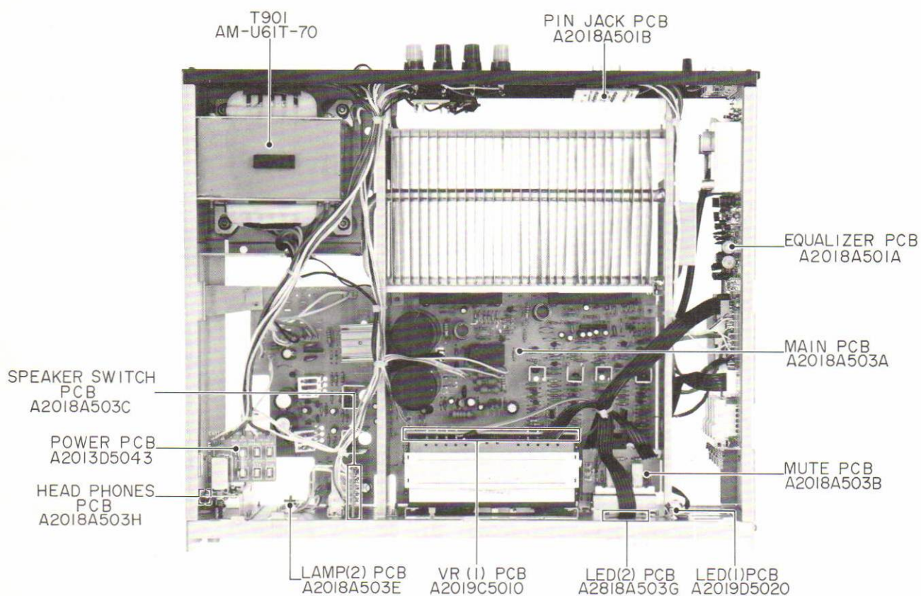
Fig. 6 Top View
