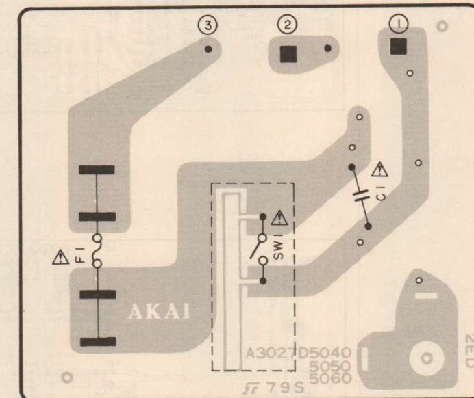
POWER PCB A3027D5060
