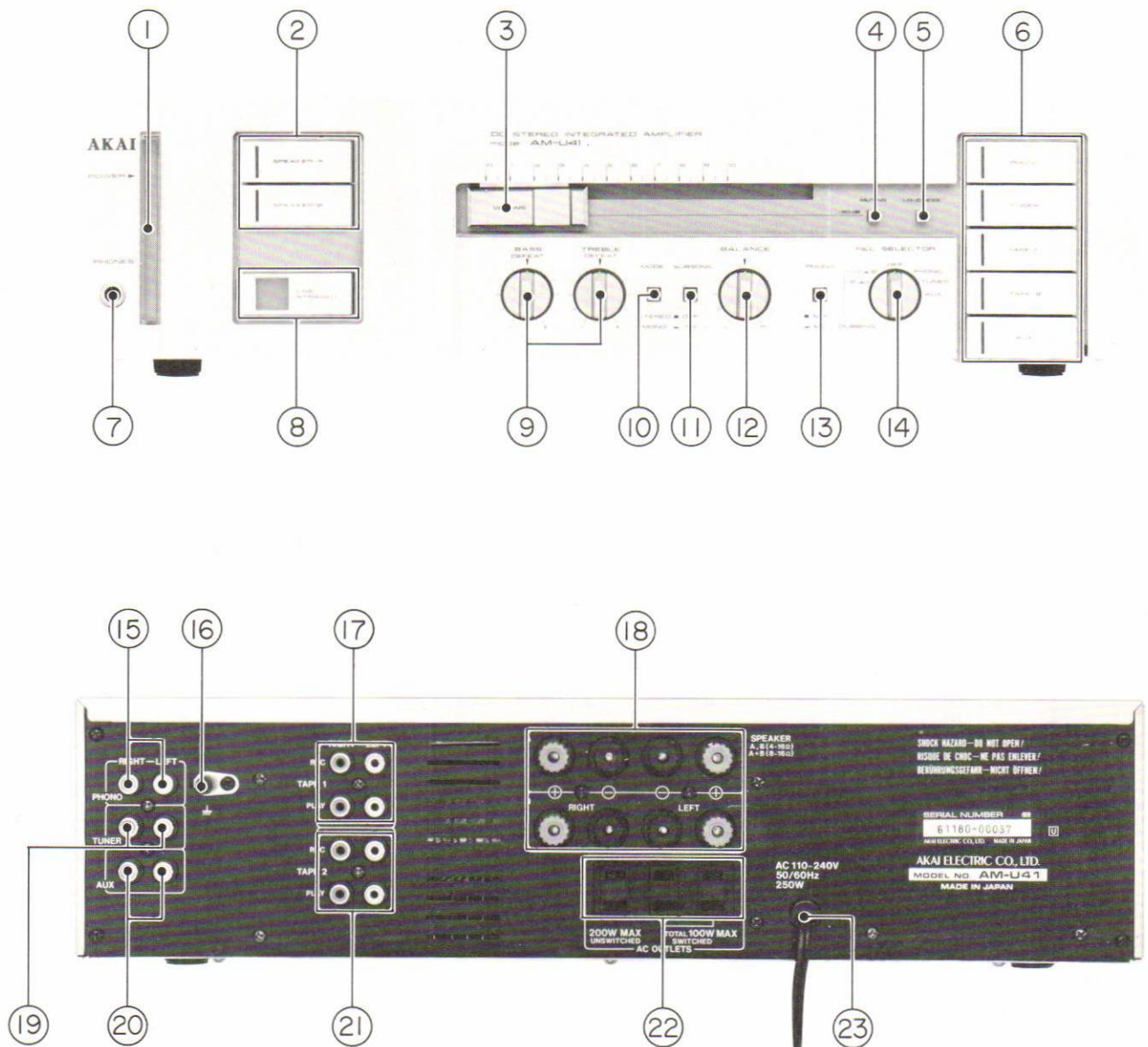
Fig. 1 Controls
