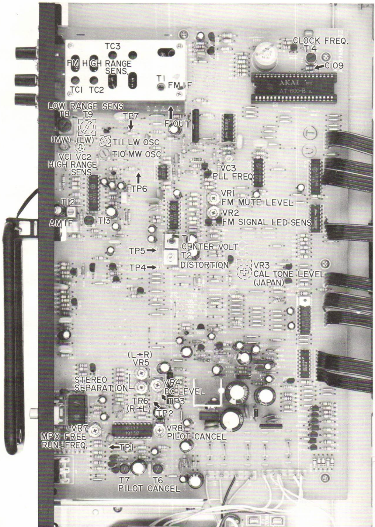
Fig. 11 Tuner P.C Board
