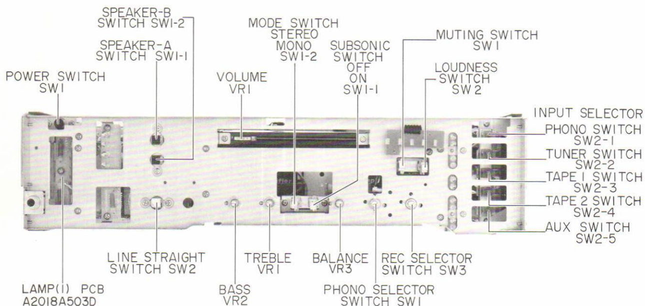
Fig. 5 Front View
