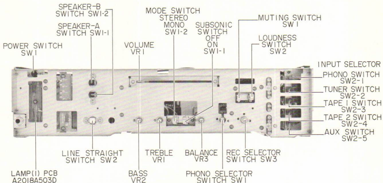
Fig. 3 Front View
