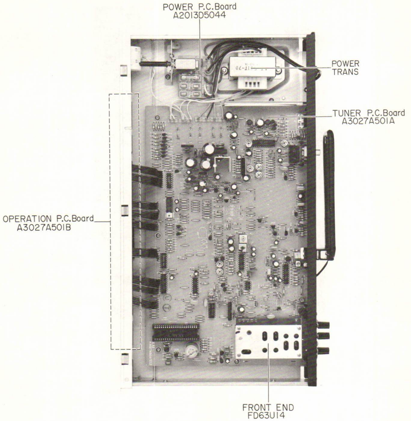
Fig. 2 Top View
