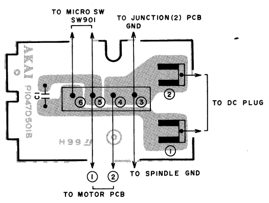
JUNCTION (1) PCB PI047D501B
