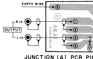
JUNCTION (A) PCB PI047D501A
