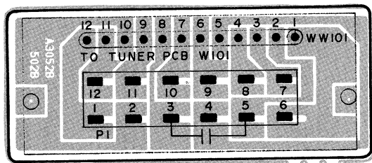
CONNECTOR PCB A3052B502B
