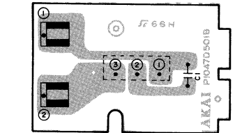
JUNCTION (B) PCB PI047D501B
