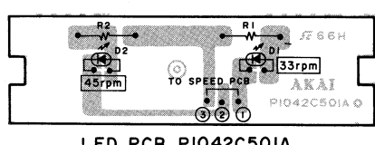
LED PCB PI042C501A
