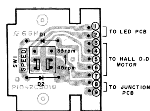
SPEED SELECTOR PCB PI042C501B
