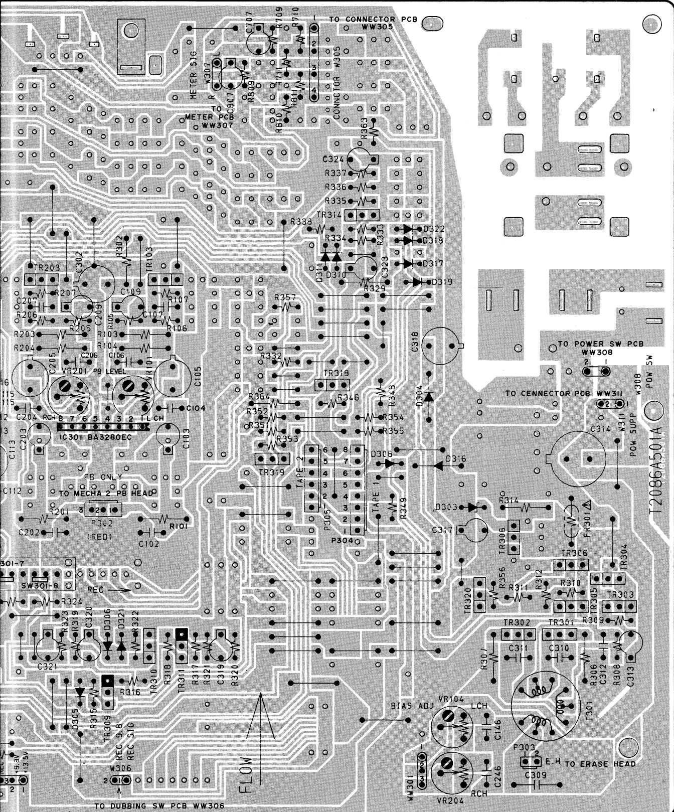
AMP PCB T2086A501A
