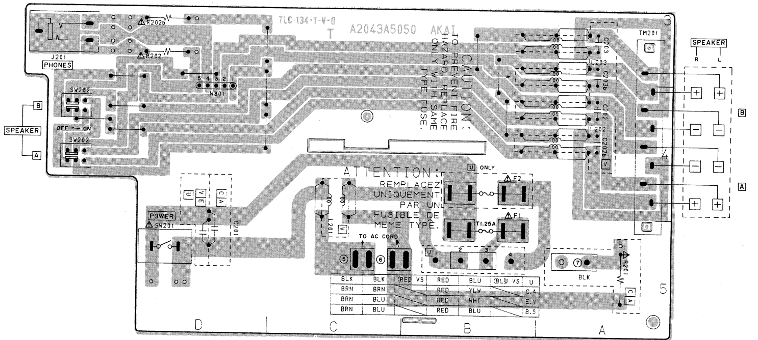
POWER SUPPLY PCB A2043A5050 5060 A.C. 5070 E.V.B.S.
