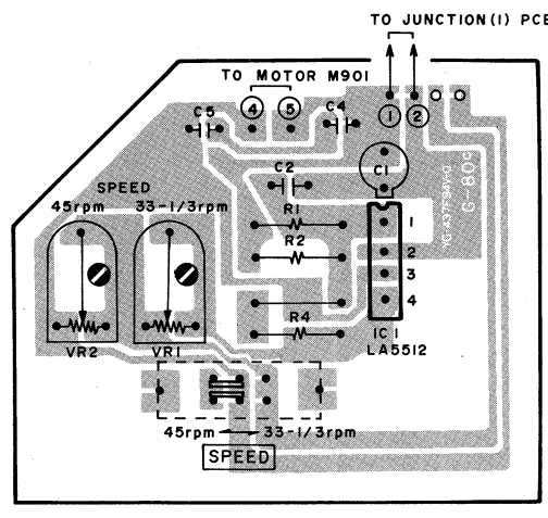
MOTOR PCB
