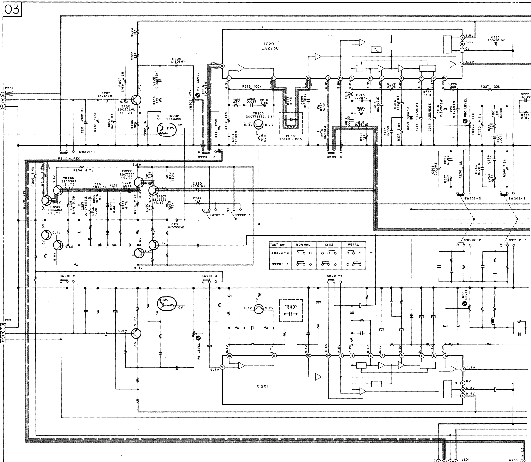
PRE AMP PCB T2085B501A
