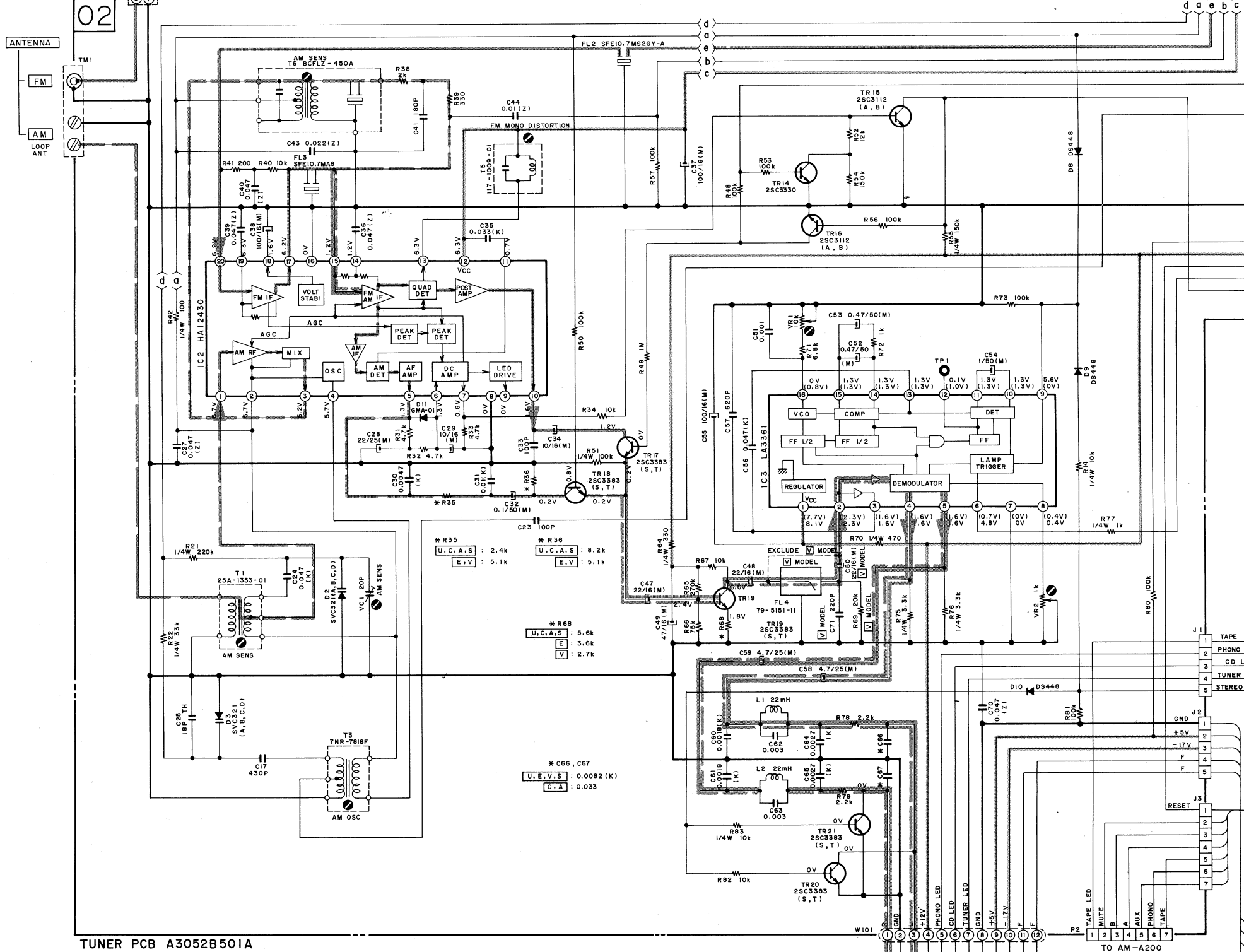
TUNER PCB A3052B501A
