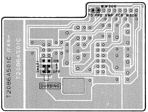
DUBBING PCB T2086A501C
