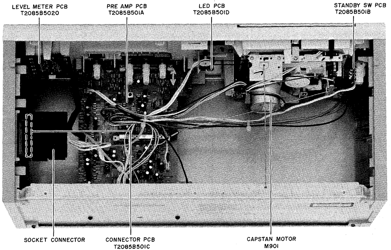
Fig. 4-1 Top View
