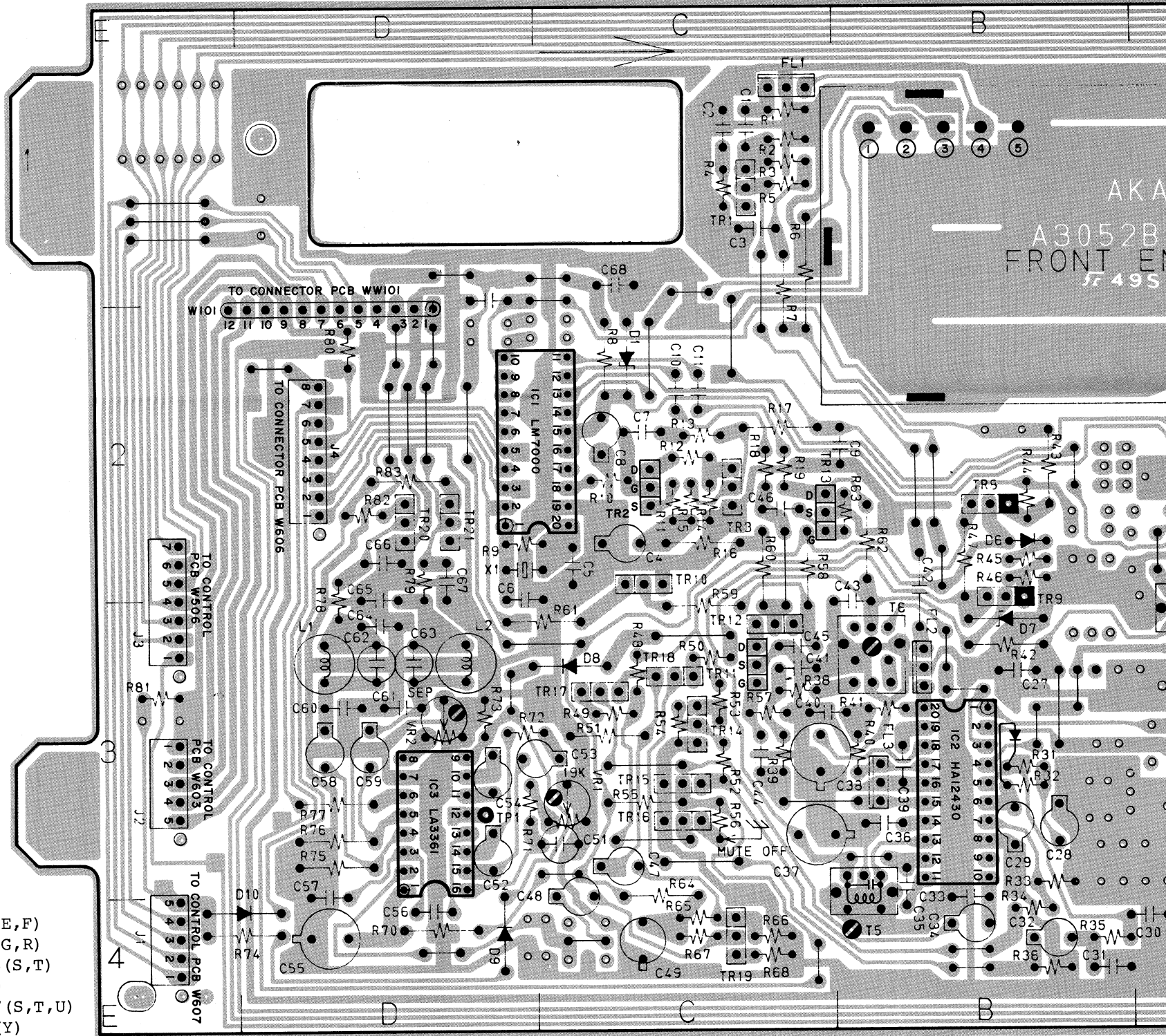
TUNER PCB A3052B501A
