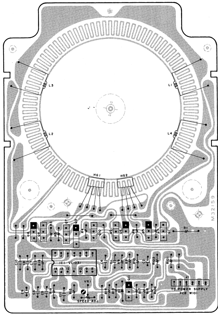
HALL D.D MOTOR M901 SS09DA
