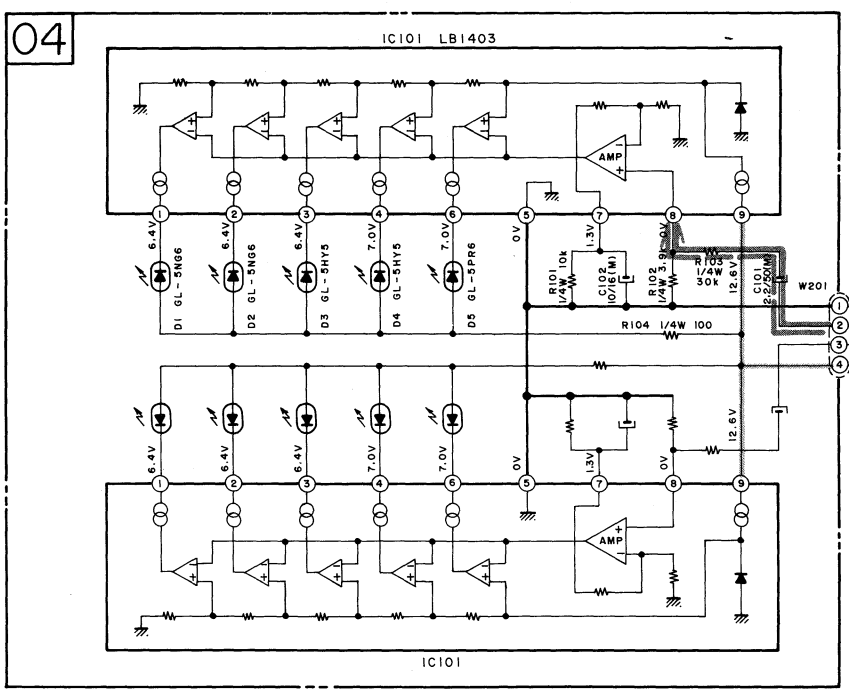
LEVEL METER PCB T2085B5020
