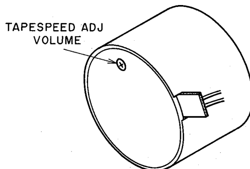
CAPSTAN MOTOR
