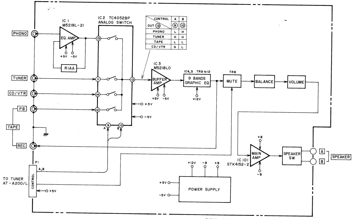
AM-A200 BLOCK DIAGRAM No. 850611A
