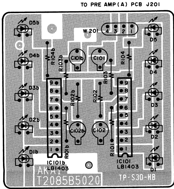
LEVEL METER PCB T2085B5020
