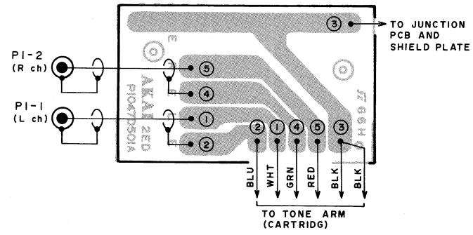
JUNCTION (2) PCB PI047D501A
