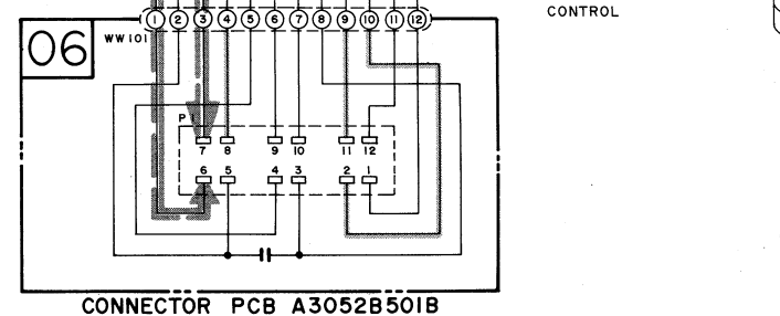
CONNECTOR PCB A3052B501B
