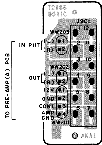
CONNECTOR PCB T2085B501C
