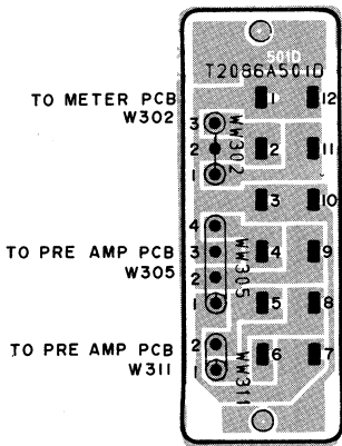
CONNECTOR PCB T2086A501D
