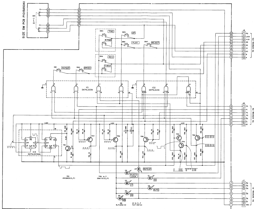
MAIN PANEL PCB P1015A5040
