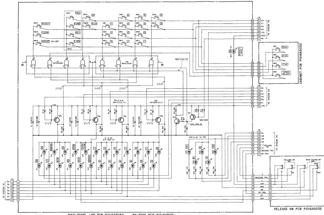
MAIN PANEL L95 PCB P1016A5030 BY-PASS PCB P1016A5031
