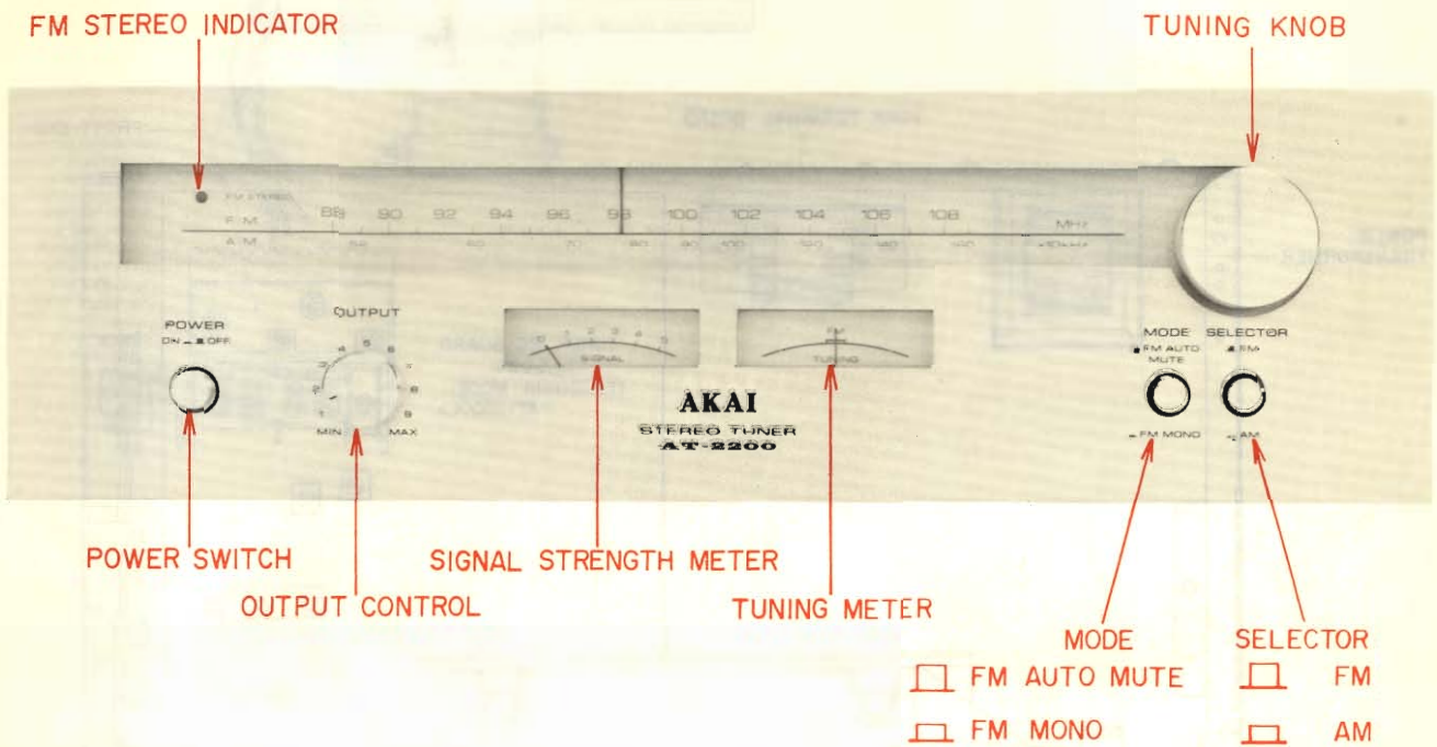
Fig. 1 Controls
