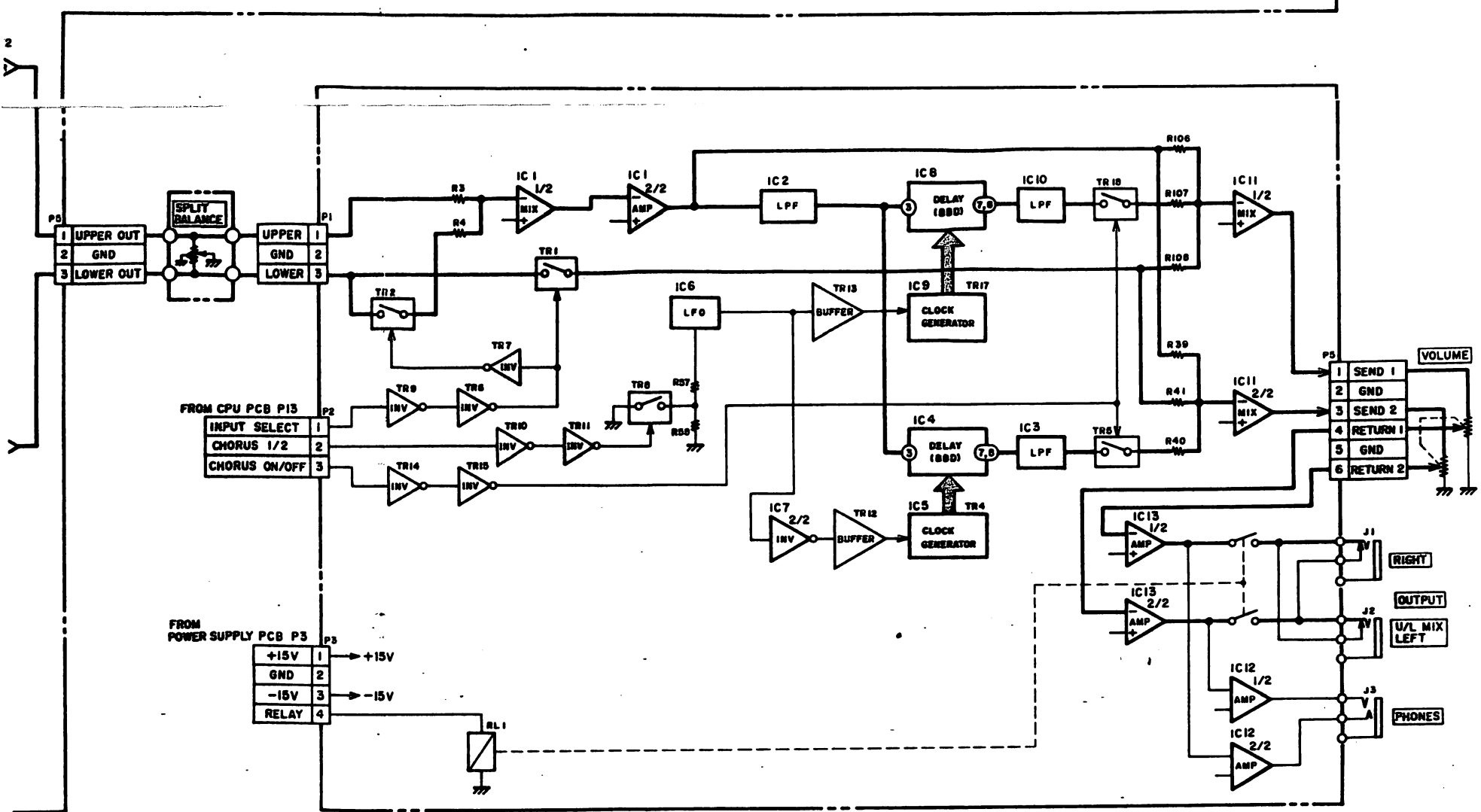
AX60 VOICE & CHORUS BLOCK DIAGRAM No.2-2 860211A
