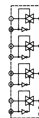
TC4066
