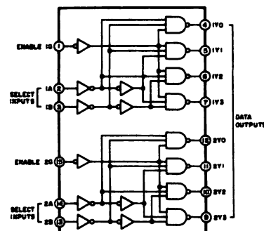
74HC139
