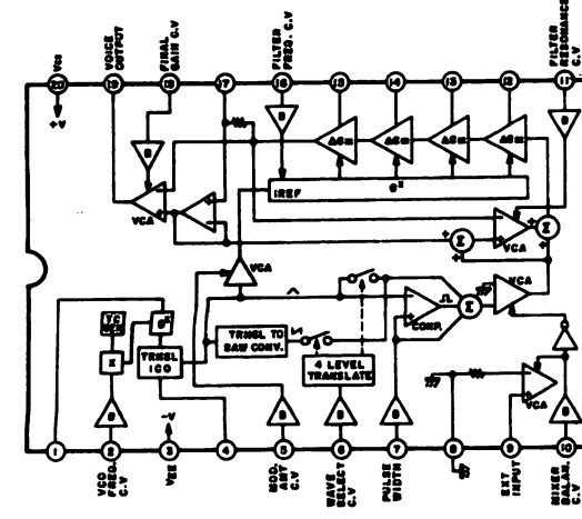
CEM3394
