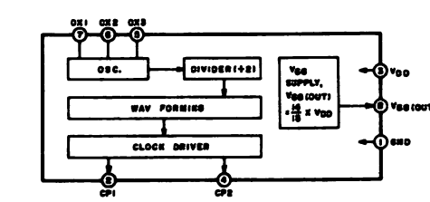
MN3101
