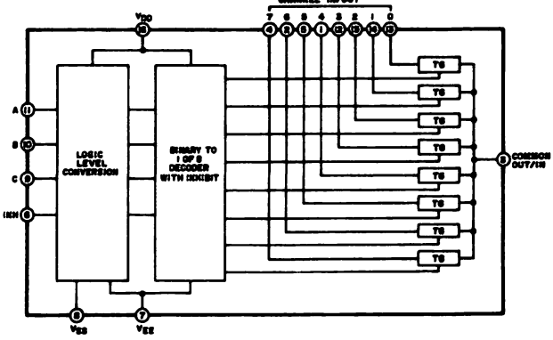
TC4051
