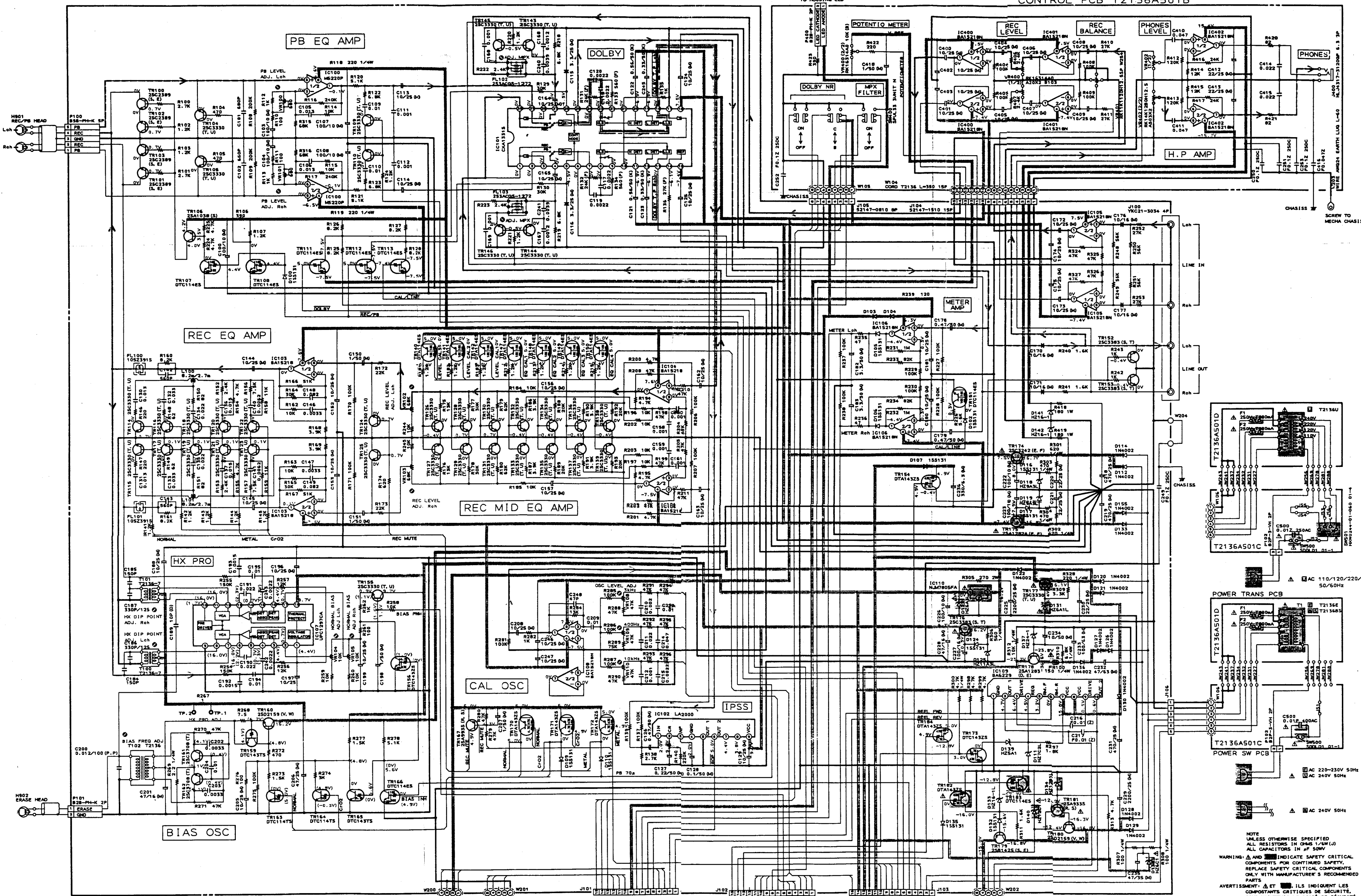
PRE AMP PCB T2136A501A
