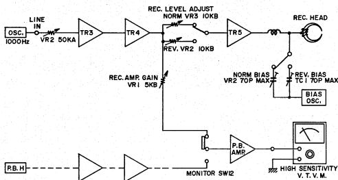
Fig. 17 REC. AMP. BLOCK DIAGRAM
