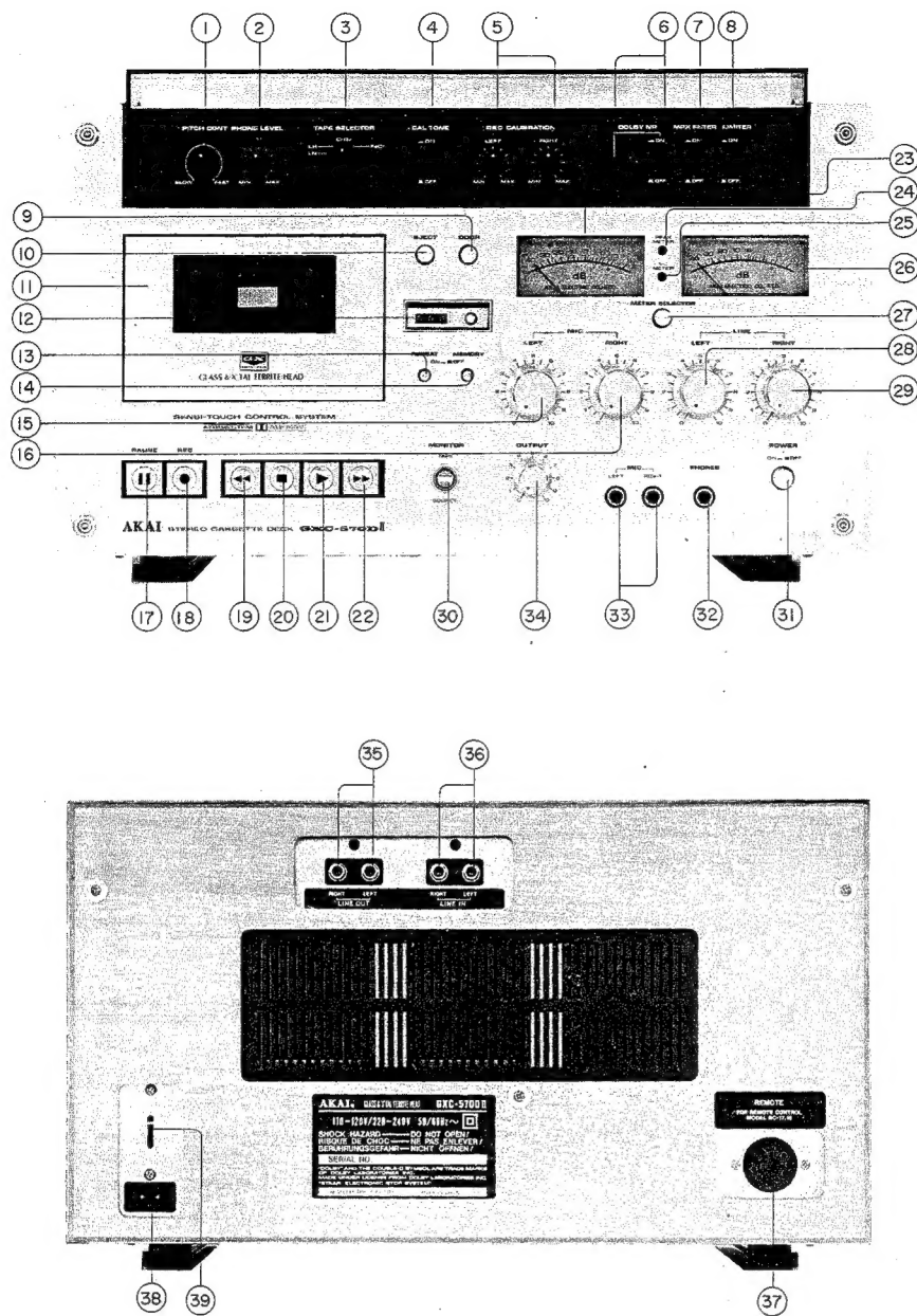
Fig. 1 Controls
