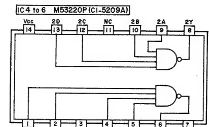
M53220P
