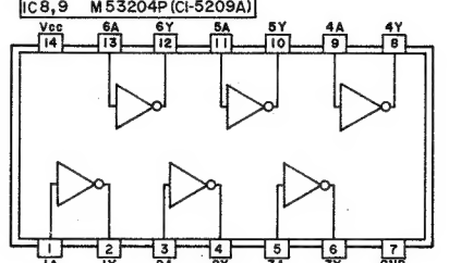
M53204P
