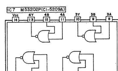
M53202P
