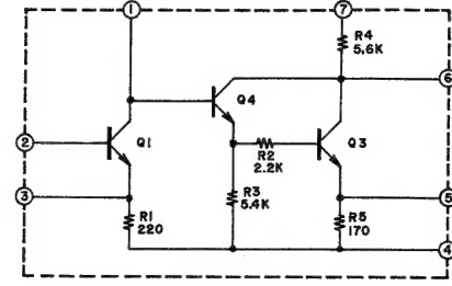
μPC1023H
