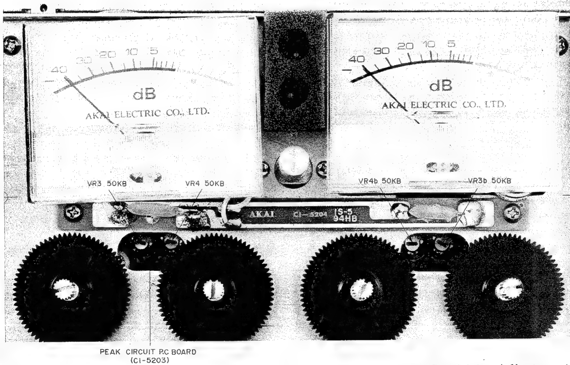
Fig. 17 Meter Sensitivity Adjustment
