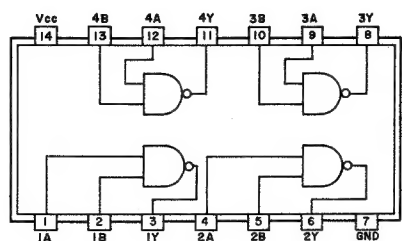
M53200P
