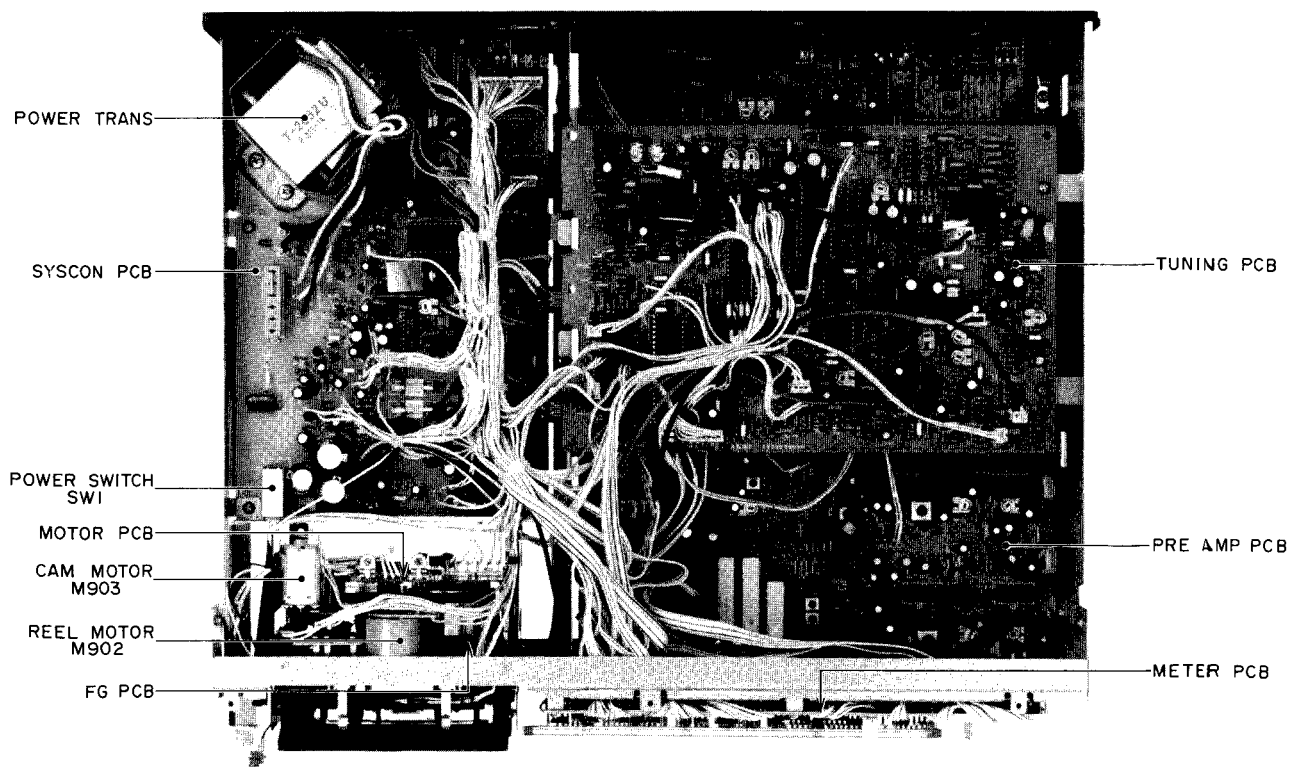
Fig. 3 Top View
