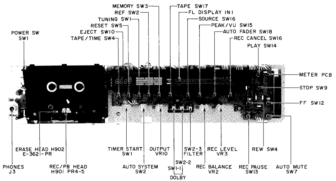
Fig. 2 Front View
