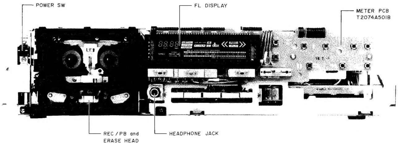
Fig. 4-1 Front View
