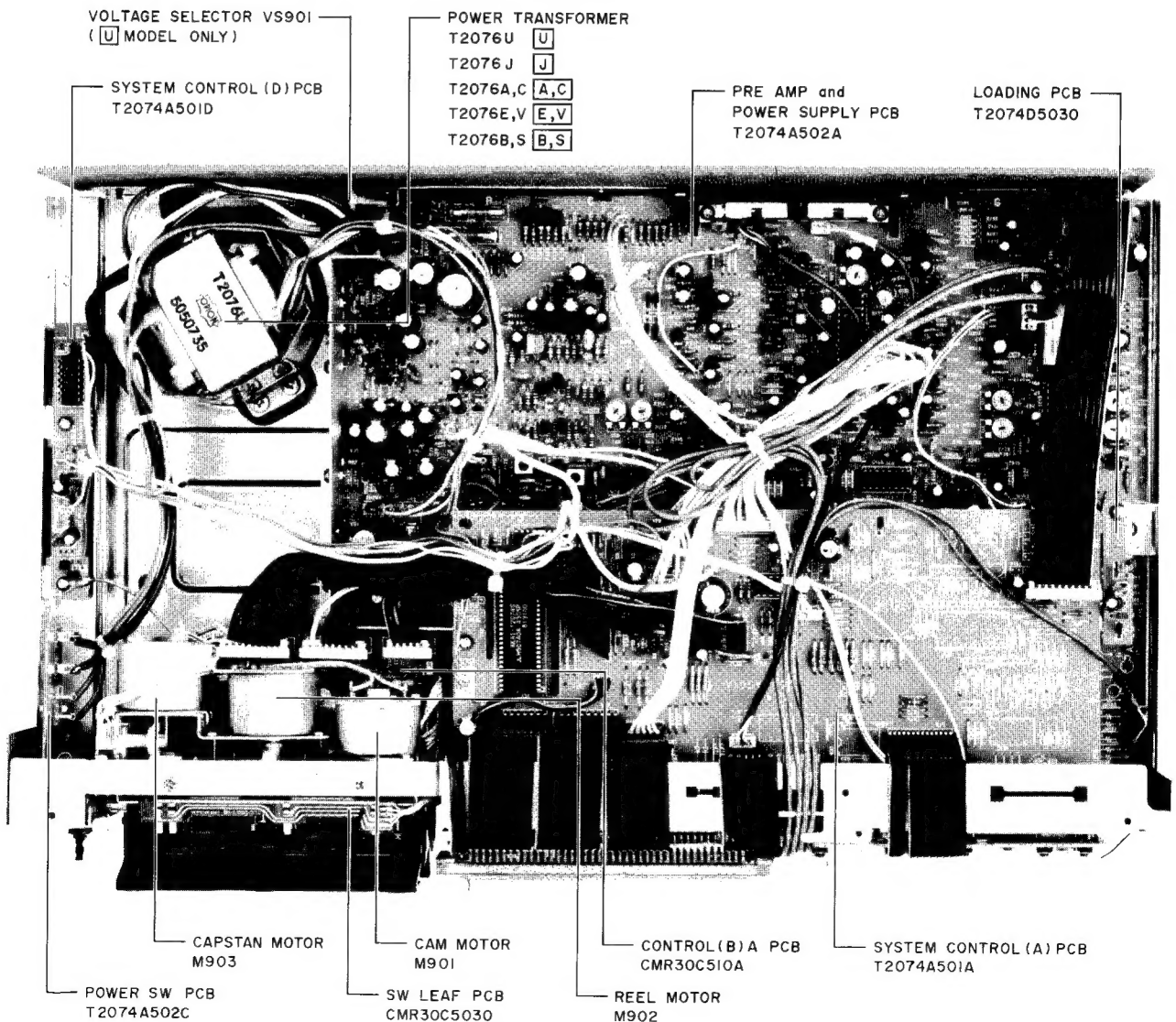
Fig. 4-2 Top View
