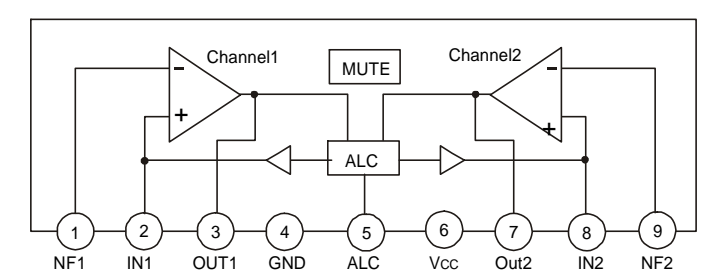
IC201 LS22241/D3308
