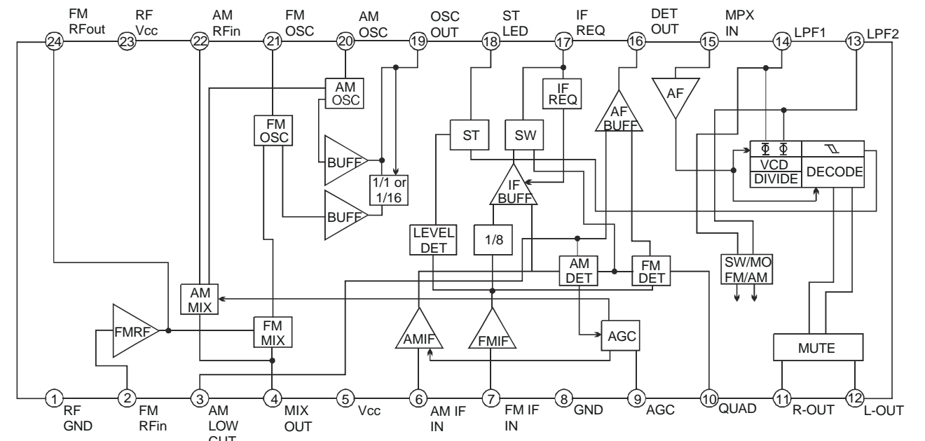
IC101 TA2149BN
