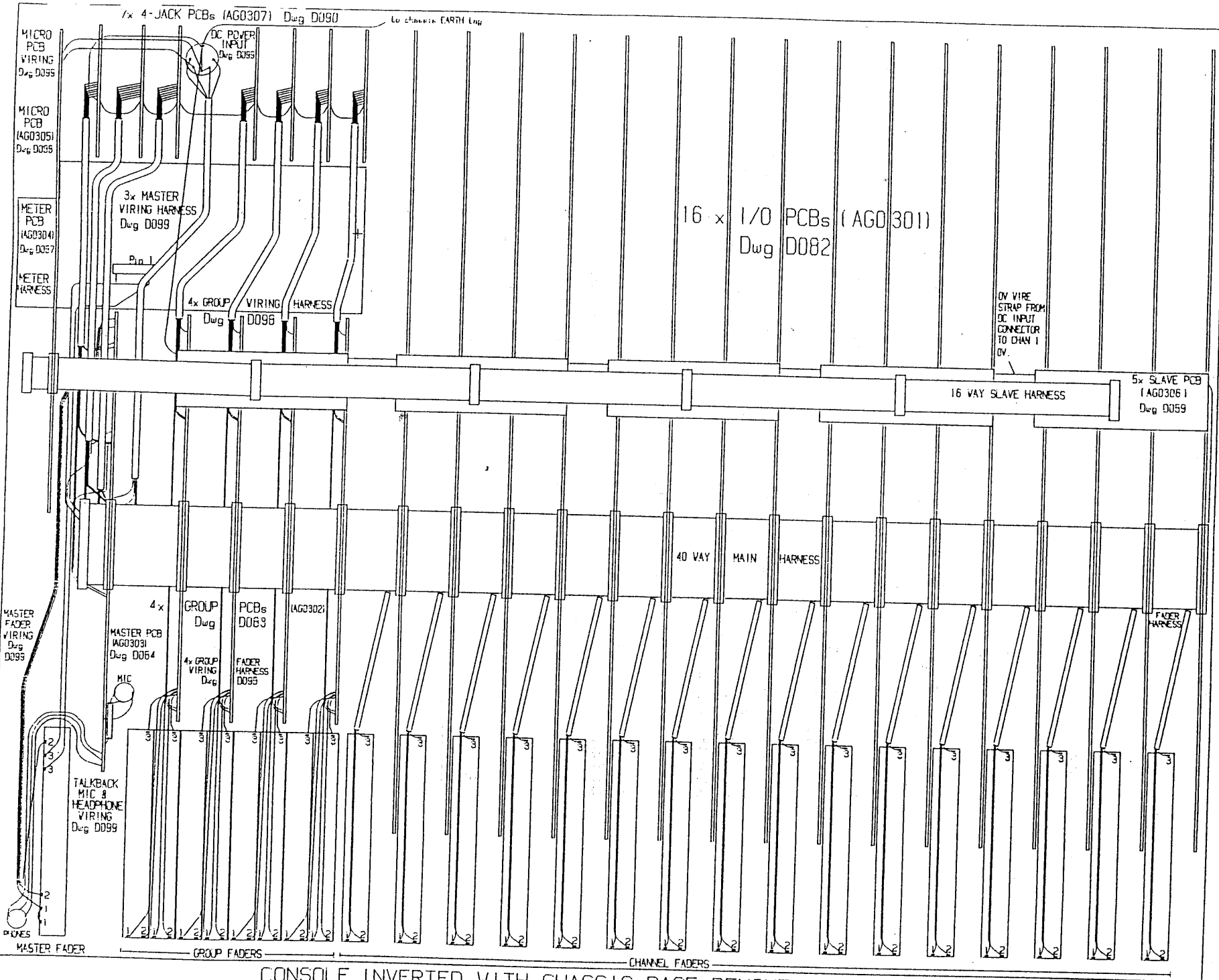
CONSOLE INVERTED WITH CHASSIS BASE REMOVED.
