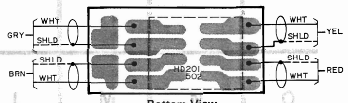
Bottom View
