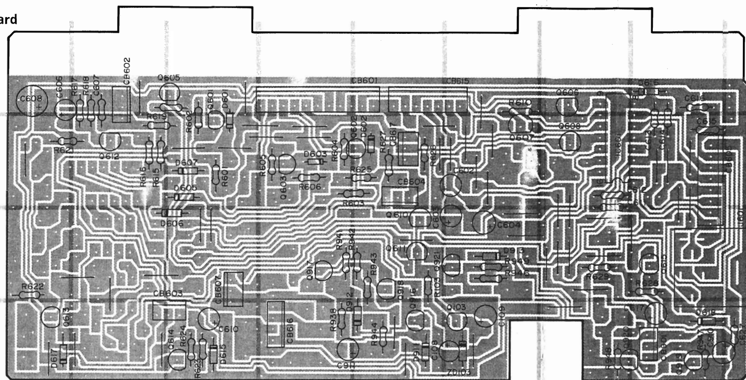
Top View
