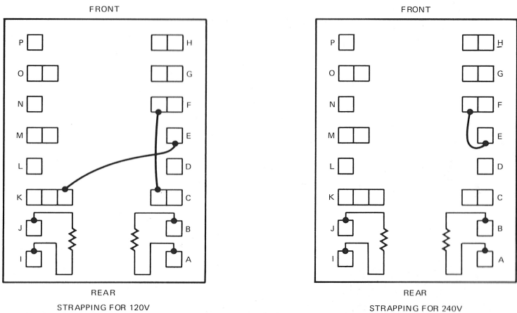
Figure 1. Strapping of Power Transformer for 120V and 240V Power
