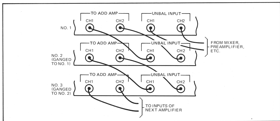
Figure 3. 9440A Amplifiers Connected in Multiple
