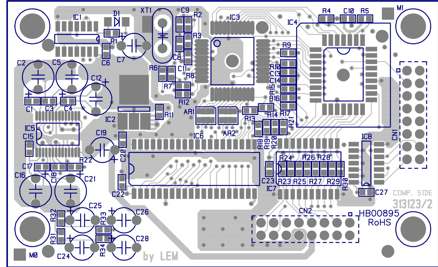
313123/2 TOP SILK RESIST COMP. SIDE
