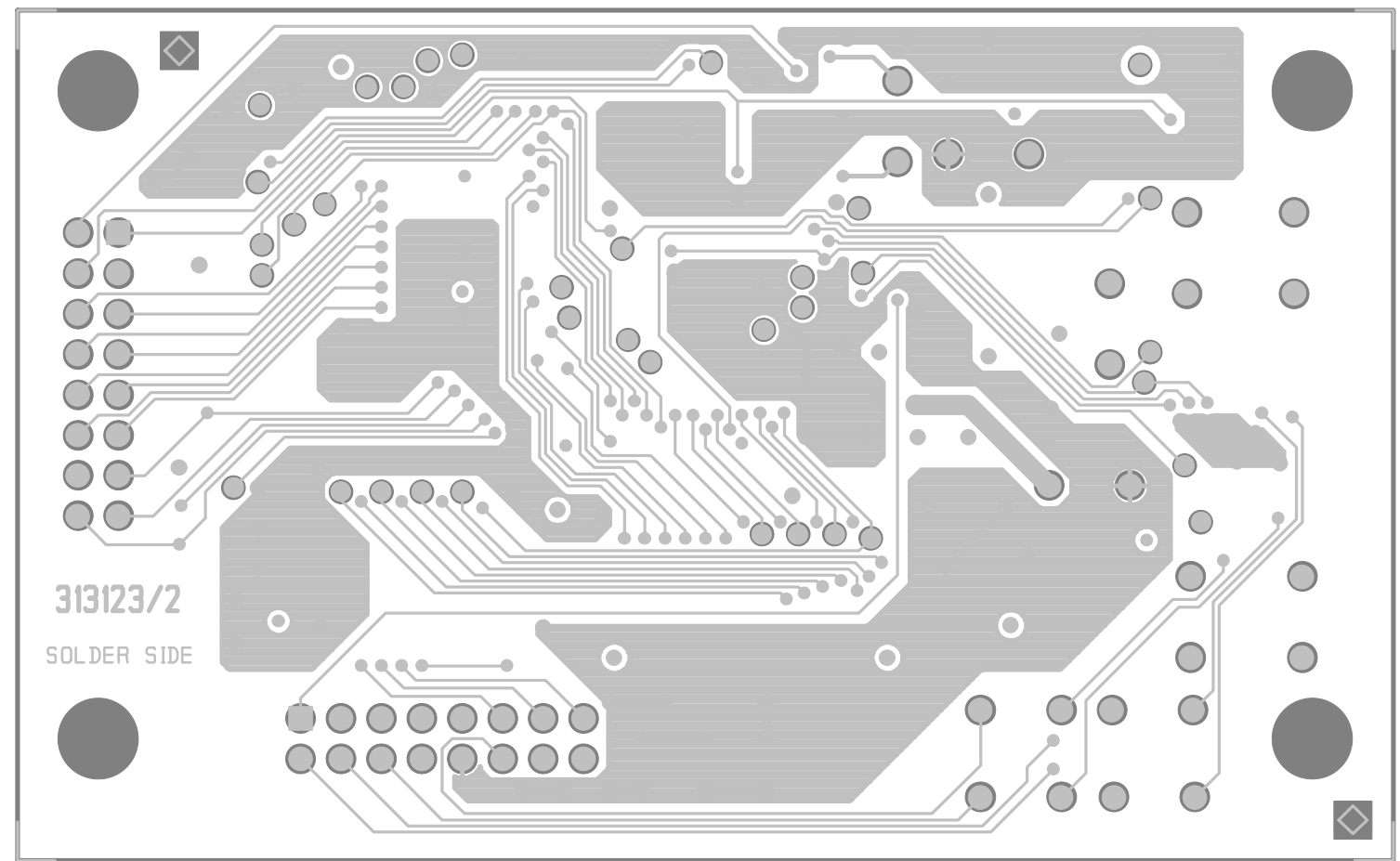
313123/2 SOLDER RESIST SOLDER SIDE
