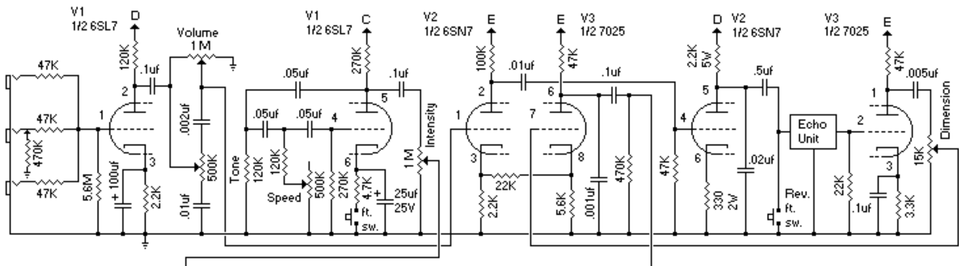
Ampeg SuperReverb Amplifier Model R-15-R Drawn by: Joe Piazza 7/31/96
