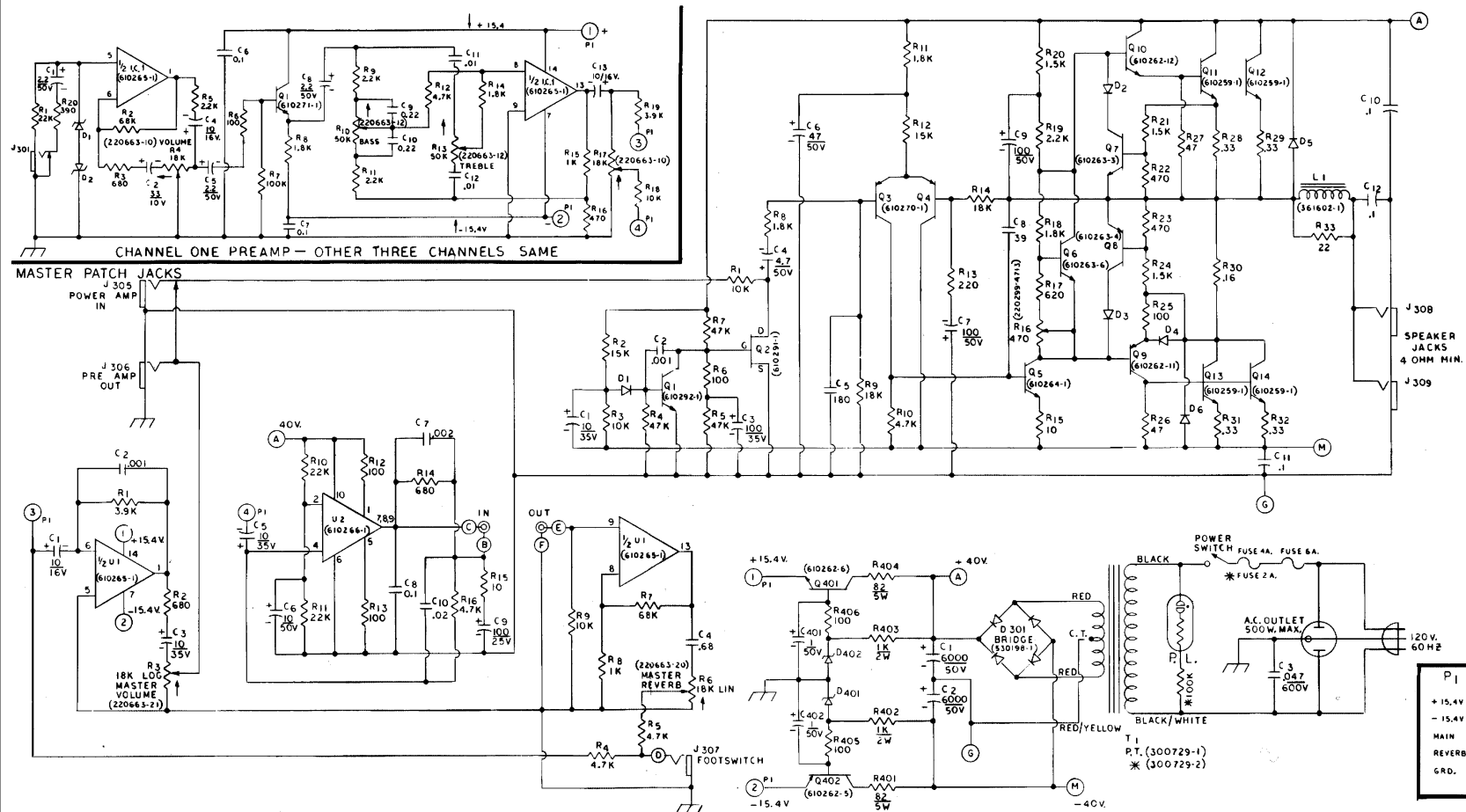
MODEL SR4 SCHEMATIC DIAGRAM
